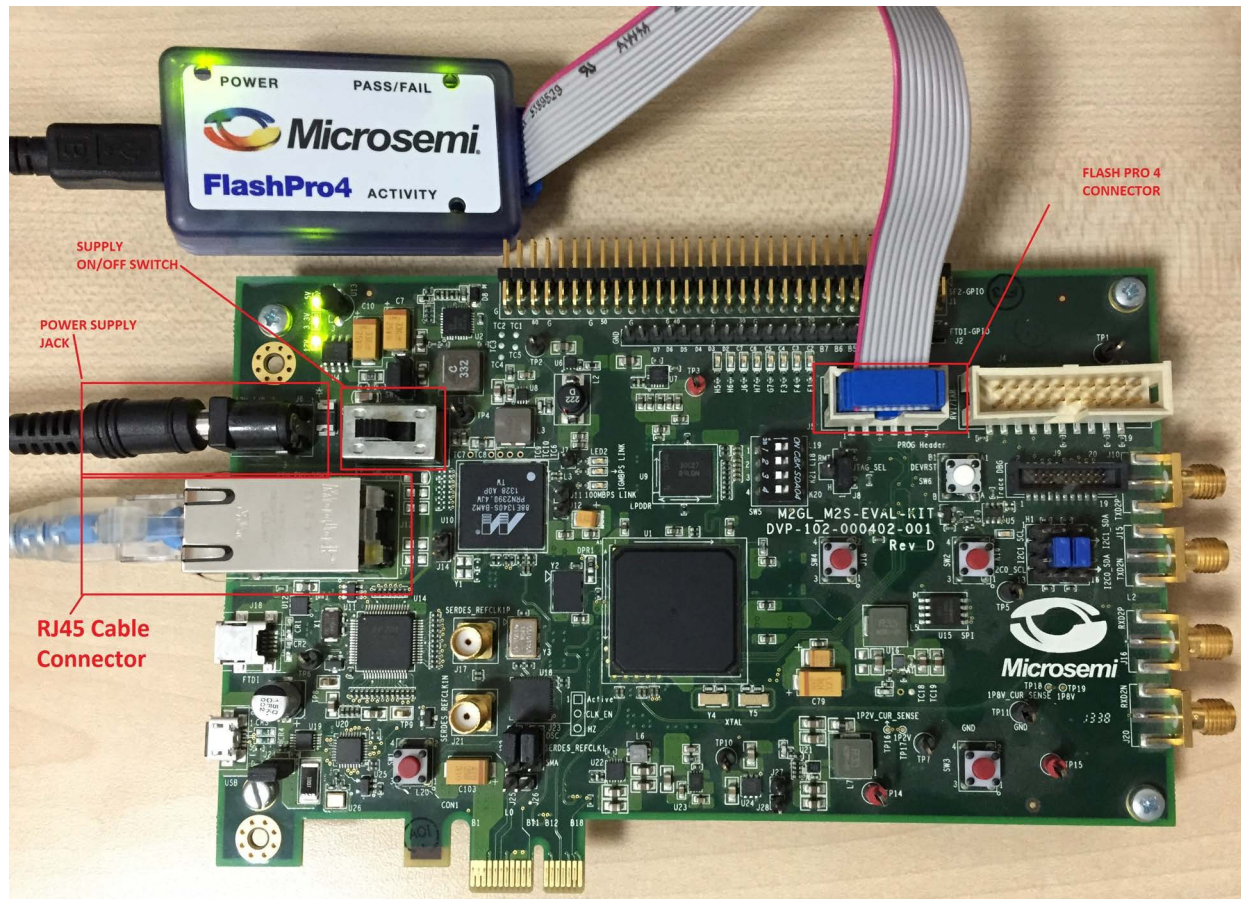
Figure 7 • SmartFusion2 Security Evaluation Kit Setup
