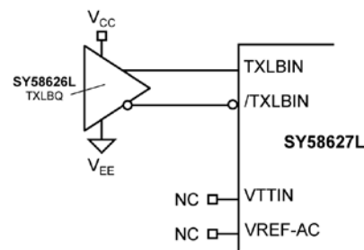
Figure 6f. TXLBIN Interface (AC-Coupled)
