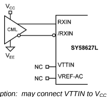
Figure 6c. CML Interface (DC-Coupled)
