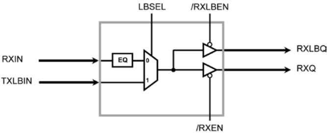
Figure 3. Loopback Control
