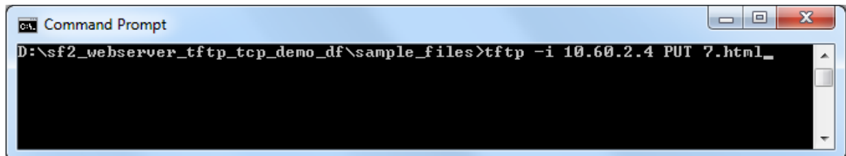
Figure 24 • Command Prompt
