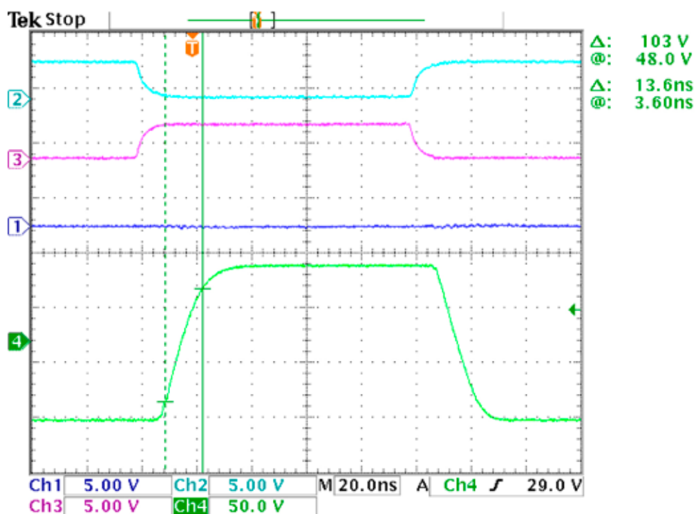
Fig 4: Input to output delay and rise time of output at V_{DD} = 10V , V_{PP}/V_{NN} = \pm 70V , Load = 330pF//2.5k, I_{OUT} = 330pF(103V/13.6ns) = 2.5A .
