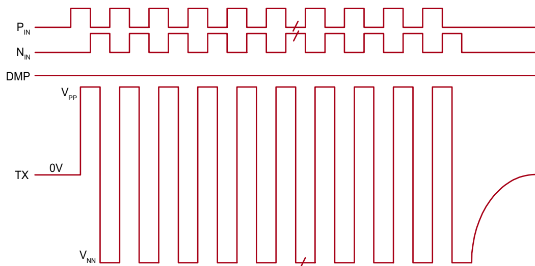
Demo Waveform E (16-Cycle w/o Damping)
