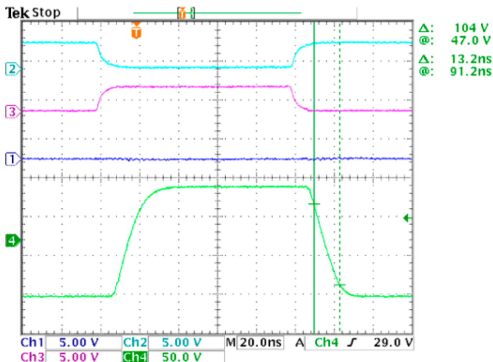
Fig 5: Input to output delay and fall time of output at V_{DD} = 10V , V_{PP}/V_{NN} = \pm 70V , Load = 330pF//2.5k, I_{OUT} = 330pF(104V/13.2ns) = 2.5A .
