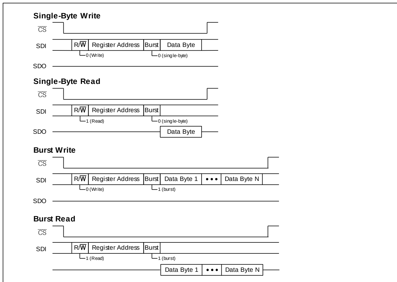
Figure 6-14. SPI Bus Transactions
