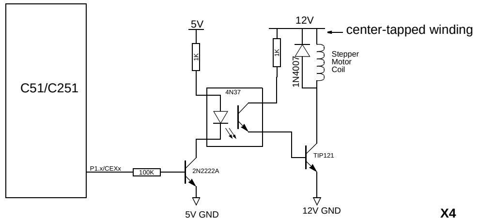
Figure 11. Power Interface
