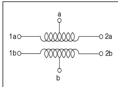
Figure 2. Unipolar Stepper Motors Coils
