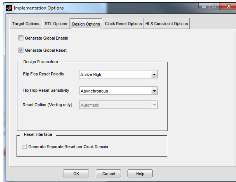
Figure 9 • Implementation Options - Design Options Tab
