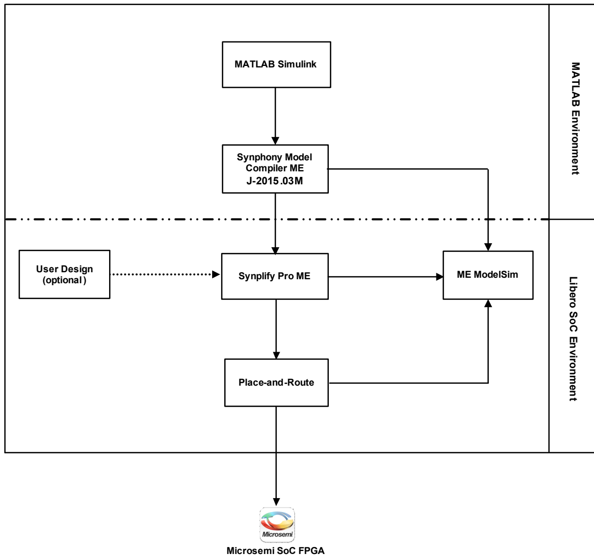
Figure 1 • DSP Design Flow
