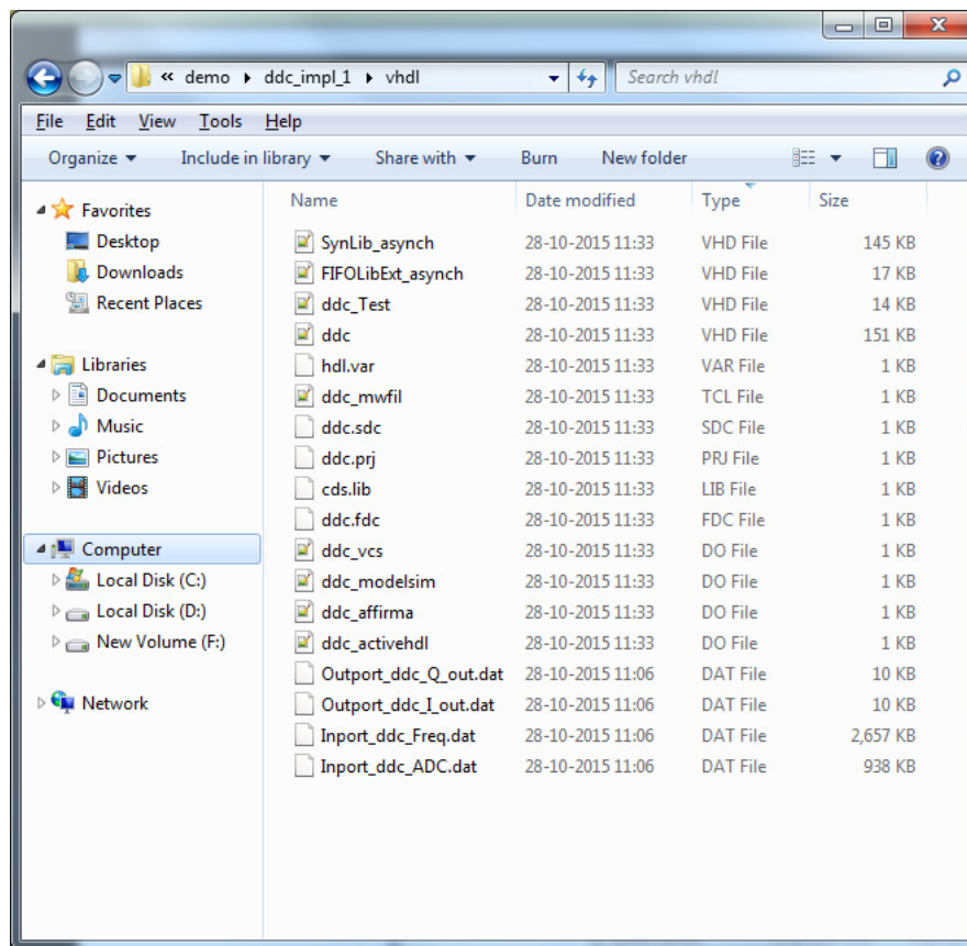
Figure 11 • VHDL Files Generated by Symphony Model Compiler ME
