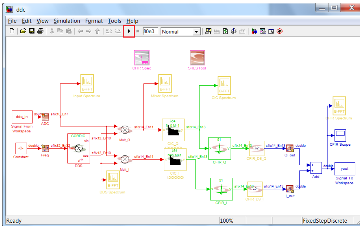
Figure 5 • DDC Design After Simulation
