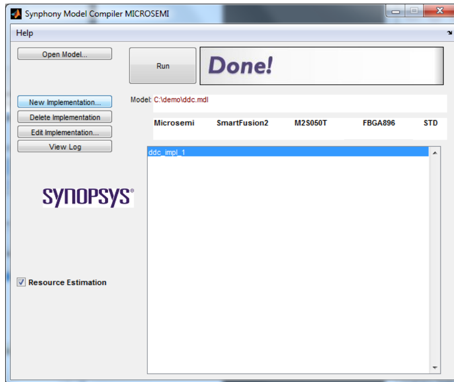
Figure 10 • Run Symphony Model Compiler
