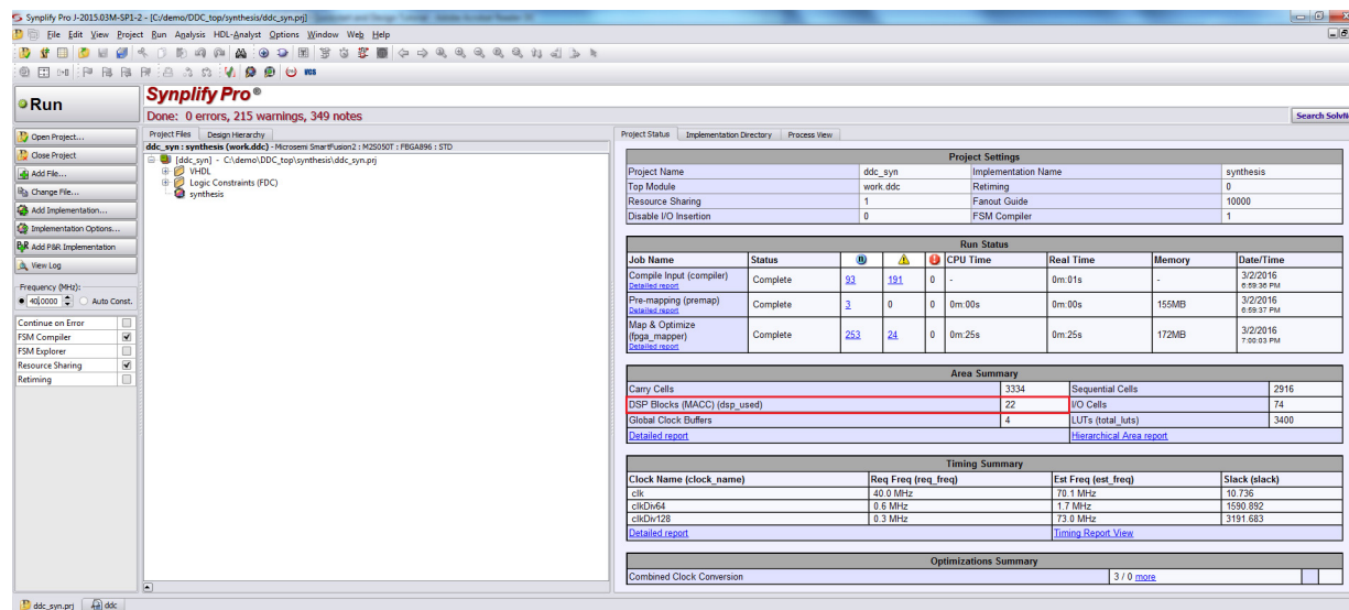
Figure 32 • Synplify Pro GUI for VHDL Flow
