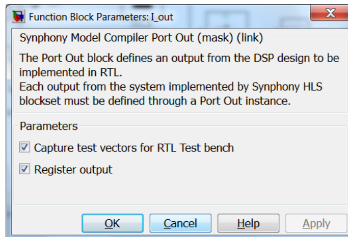
Figure 4 • Setting the Output Port I_out
