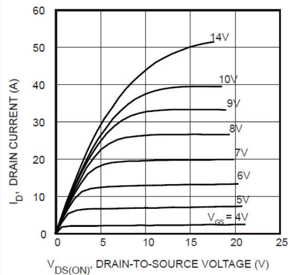
Figure 1-1. Output Characteristics
