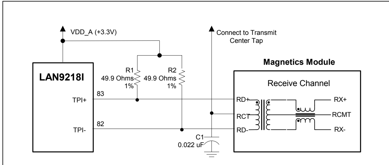
Figure 2.2 Receive Circuit
