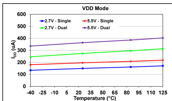
FIGURE 2-4: Average Device Supply Current - Inactive Interface ( SCK = V_{IH} or V_{IL} ) vs. Voltage and Temperature, VRxB:VRxA = '00' ( V_{DD} Mode).
