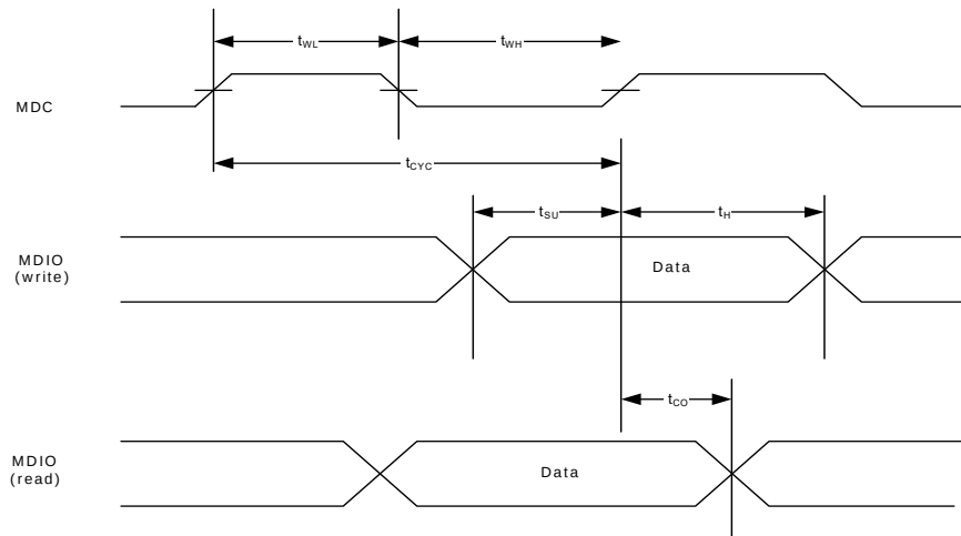
Figure 80 • Serial Management Interface Timing
