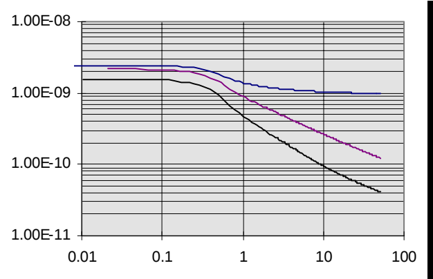
Figure 1 Device A: Ciss, Coss, Crss vs. Vds
