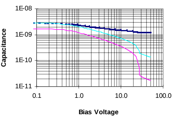
Figure 2 Device B: Ciss, Coss, Crss vs. Vds
