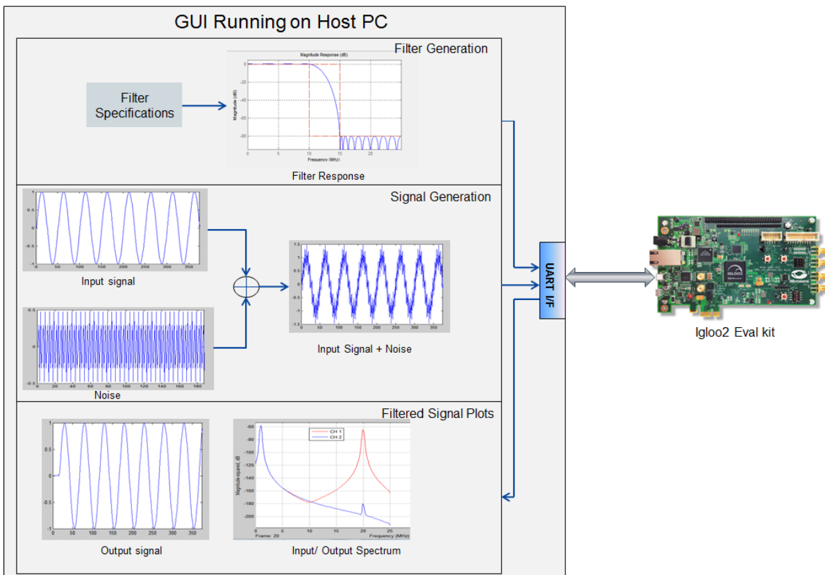
Figure 1 • Top-Level Diagram of DSP FIR Filter Demo
