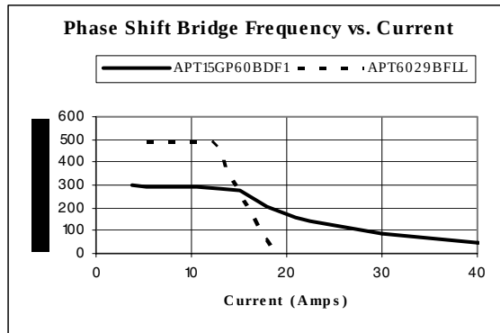
Figure 7 Phase Shift Bridge Frequency vs. Current
