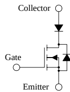
Figure 2 Simple IGBT Equivalent Circuit
