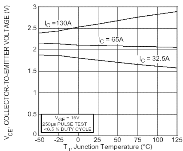
Figure 5 V_{CE(on)} TC for APT65GP60B2
