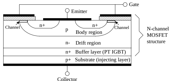
Figure 1 PT IGBT Cross Section
