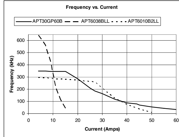
Figure 4 Usable Frequency vs. Current
