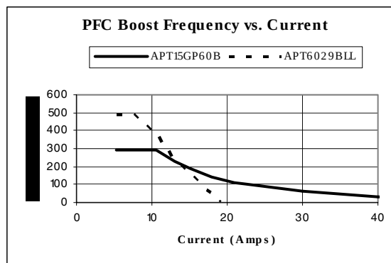
Figure 6 PFC Boost Frequency vs. Current
