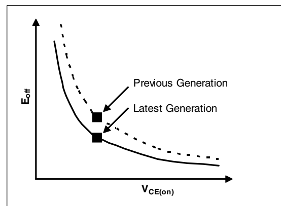
Figure 3 Turn-Off Energy vs. V_{CE(on)}
