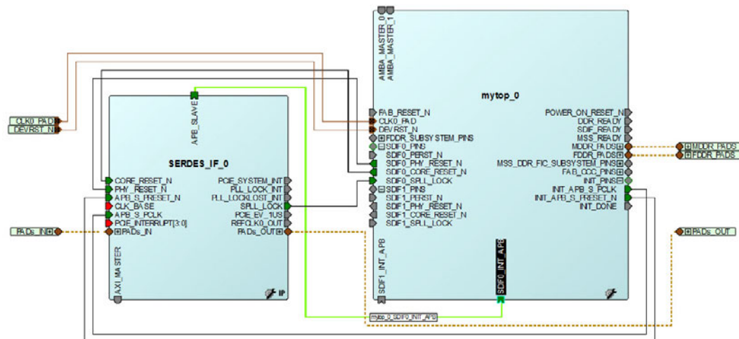
Figure 2-7 • SERDESIF Peripheral Initialization Connectivity
