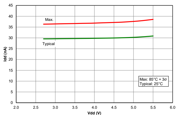
Figure 39-64. I_{PD} , Fixed Voltage Reference (FVR), PIC18F26/45/46K40 only
