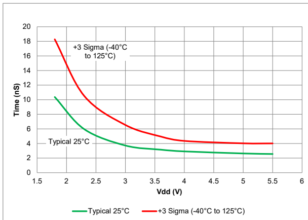
Figure 39-60. I/O Fall Time, Slew Rate Control Disabled
