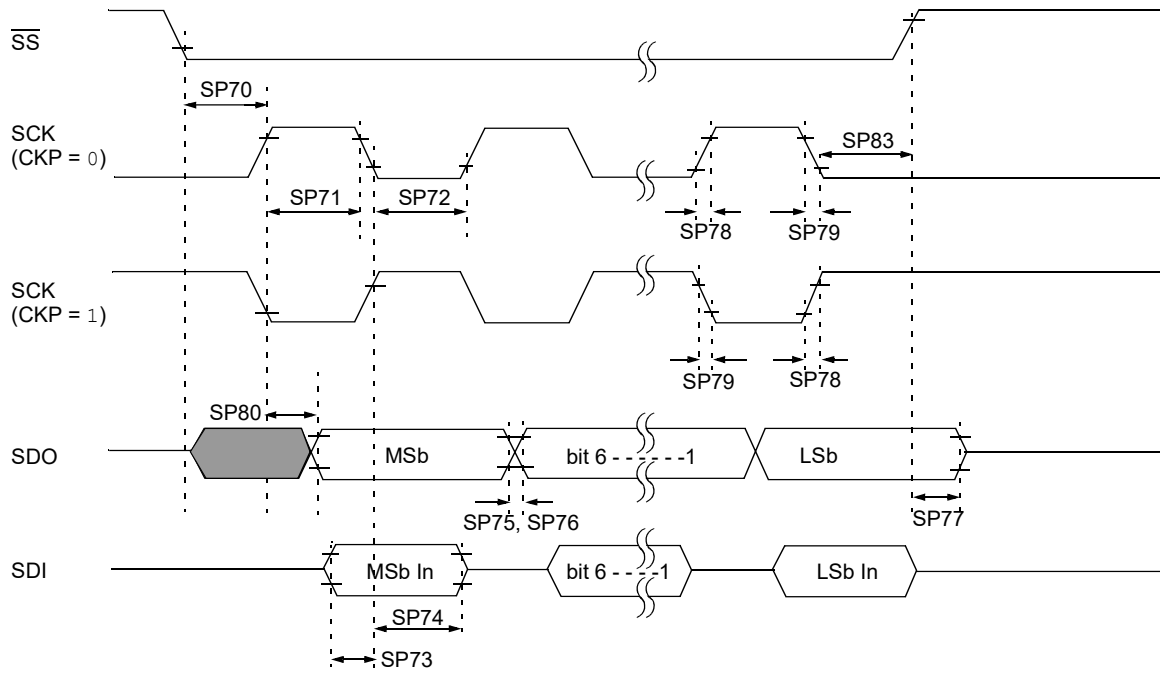
Figure 38-18. SPI Client Mode Timing (CKE = 0)
