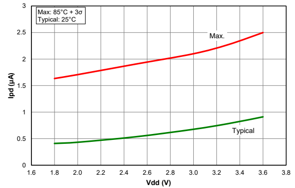
Figure 39-61. I_{PD} , Watchdog Timer, PIC18LF26/45/46K40 only
