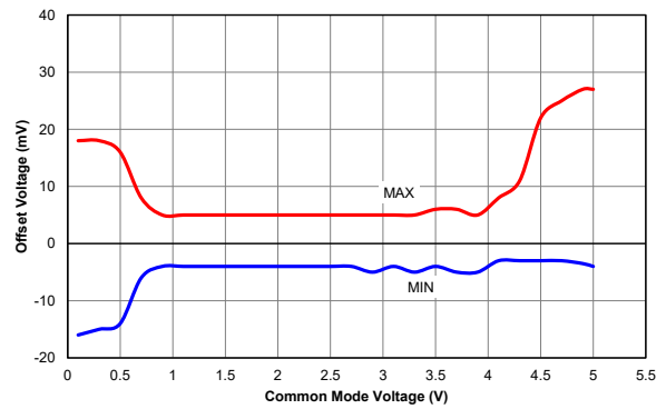
Figure 39-33. Comparator Offset, V_{DD} = 5.5V , -40°C to 125°C, PIC18F26/45/46K40 only
