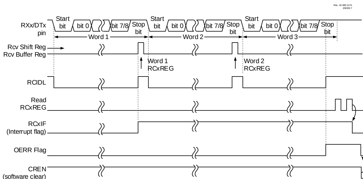
Figure 28-5. Asynchronous Reception
