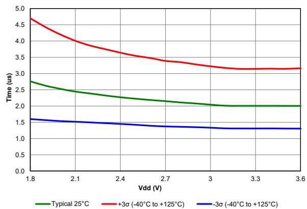
Figure 39-9. ADC RC Oscillator Period, PIC18LF26/45/46K40 only
