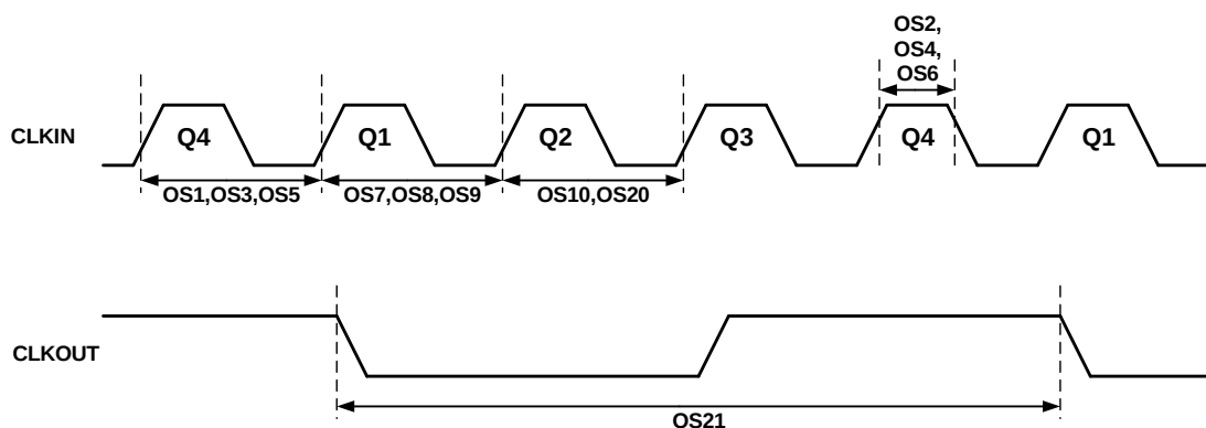
Figure 38-5. Clock Timing
