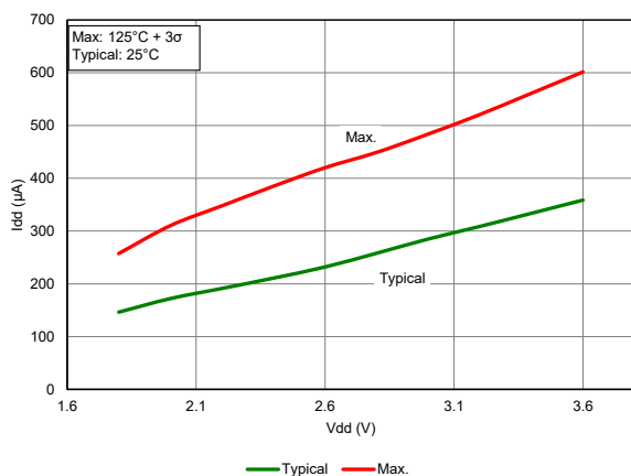
Figure 39-50. I_{DD} , ECM Oscillator, F_{OSC} = 4 MHz, PIC18LF26/45/46K40 only
