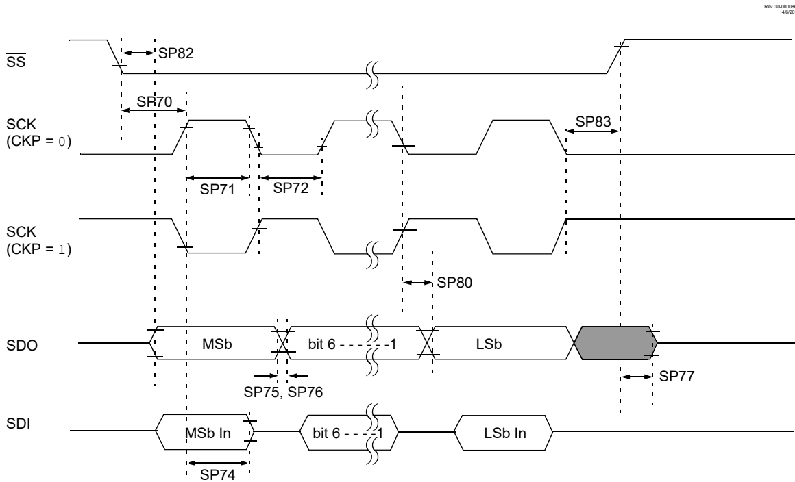
Figure 38-19. SPI Client Mode Timing (CKE = 1)
