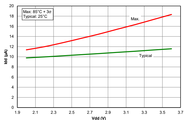
Figure 39-65. I_{PD} , Brown-out Reset, BORV = 1, PIC18LF26/45/46K40 only
