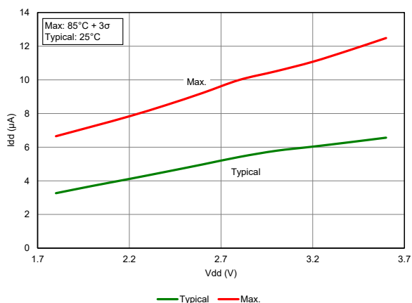
Figure 39-48. I_{DD} , LFINTOSC, F_{OSC} = 31 kHz, PIC18LF26/45/46K40 only
