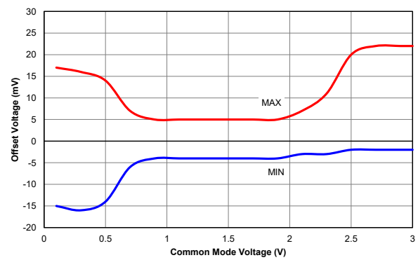
Figure 39-29. Comparator Offset, V DD = 3.0V, -40°C to 125°C
