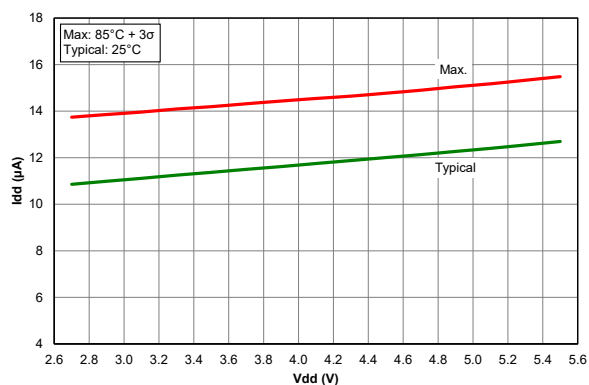
Figure 39-66. I_{PD} , Brown-out Reset, BORV = 1, PIC18F26/45/46K40 only
