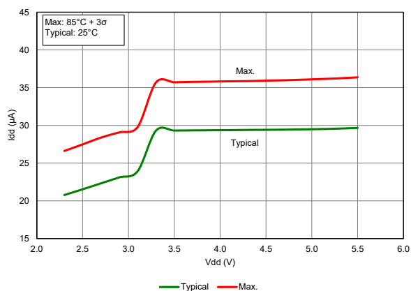
Figure 39-42. I_{DD} , LFINTOSC, F_{OSC} = 31 kHz, PIC18F26/45/46K40 only
