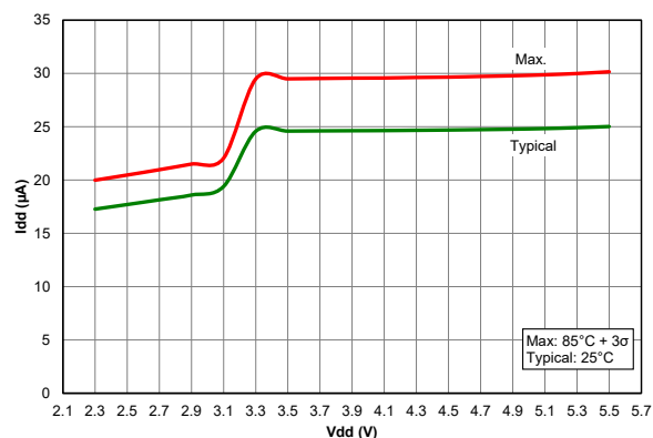
Figure 39-73. I_{PD} Base, VREGPM = 01, PIC18F26/45/46K40 only
