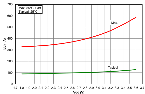
Figure 39-67. I_{PD} , Low-power Brown-out Reset, LPBOR = 0, PIC18LF26/45/46K40 only
