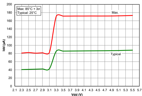
Figure 39-72. I_{PD} Base, VREGPM = 00, PIC18F26/45/46K40 only
