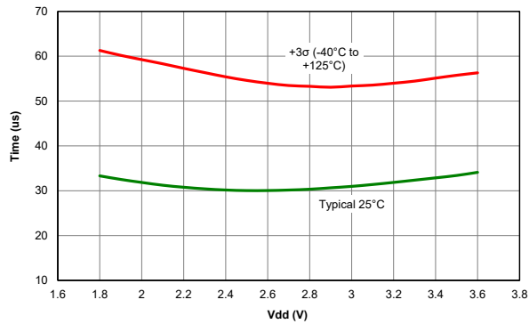
Figure 39-11. Bandgap Ready Time, PIC18LF26/45/46K40
