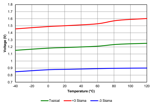
Figure 39-81. POR Rearm Voltage, VREGPM1 = 1, PIC18F26/45/46K40 only
