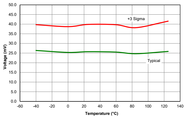
Figure 39-21. Brown-Out Reset Hysteresis, Trip Point (BORV = 1.1), PIC18LF26/45/46K40 only
