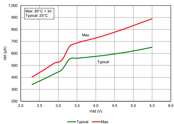
Figure 39-44. I_{DD} , ECM Oscillator, F_{OSC} = 4 MHz, PIC18F26/45/46K40 only
