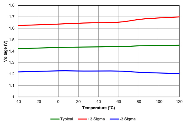
Figure 39-80. POR Rearm Voltage, VREGPM1 = 0, PIC18F26/45/46K40 only
