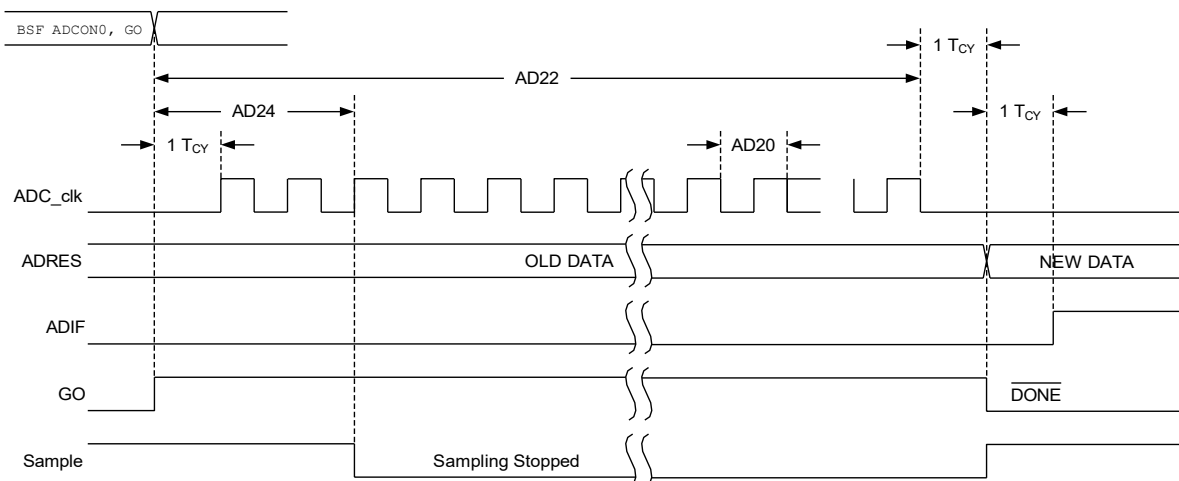
Figure 38-10. ADC Conversion Timing (ADC Clock F_{OSC} -Based)
