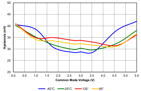
Figure 39-31. Comparator Hysteresis, V_{DD} = 5.5V , PIC18F26/45/46K40 only
