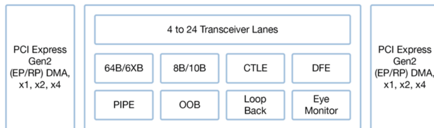
Figure 10 Transceiver Architecture and Features
