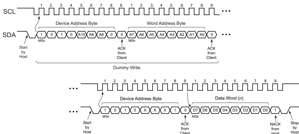
Figure 8-2. Random Read
