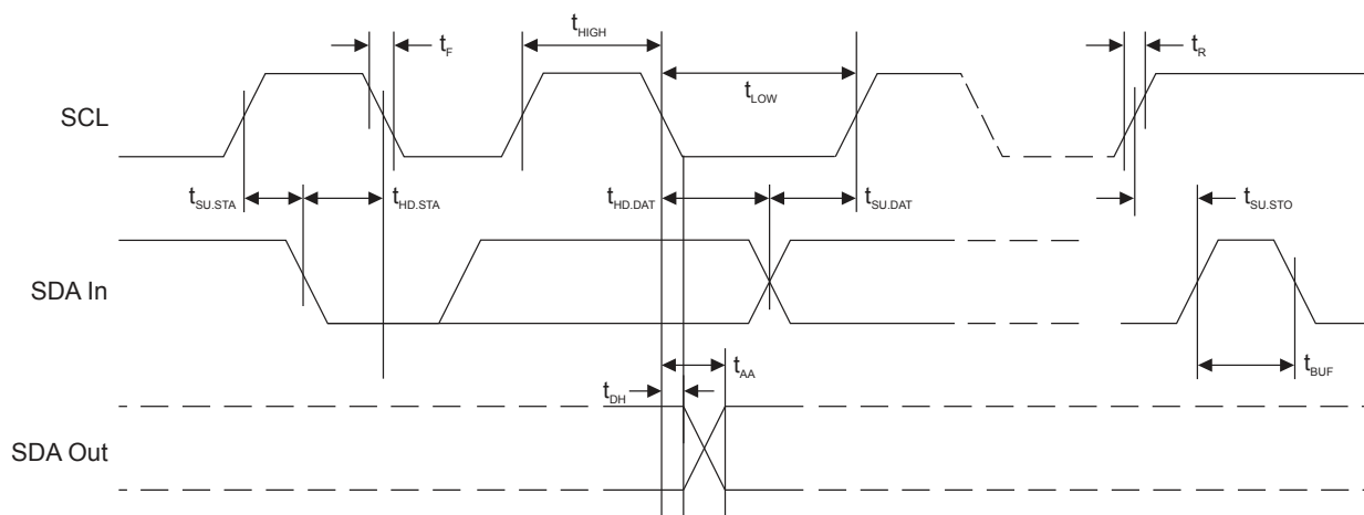
Figure 4-1. Bus Timing
