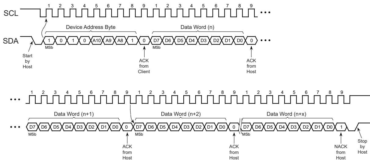
Figure 8-3. Sequential Read
