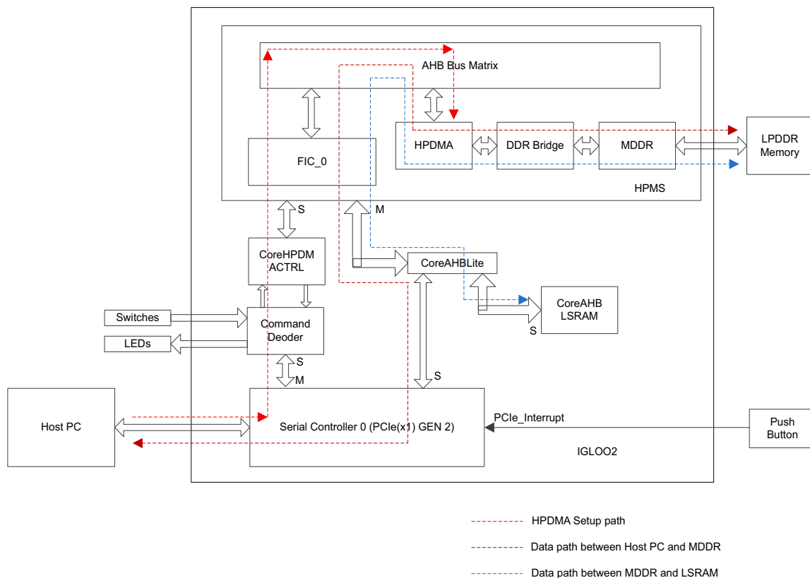
Figure 2 • PCIe Data Plane Demo Block Diagram
