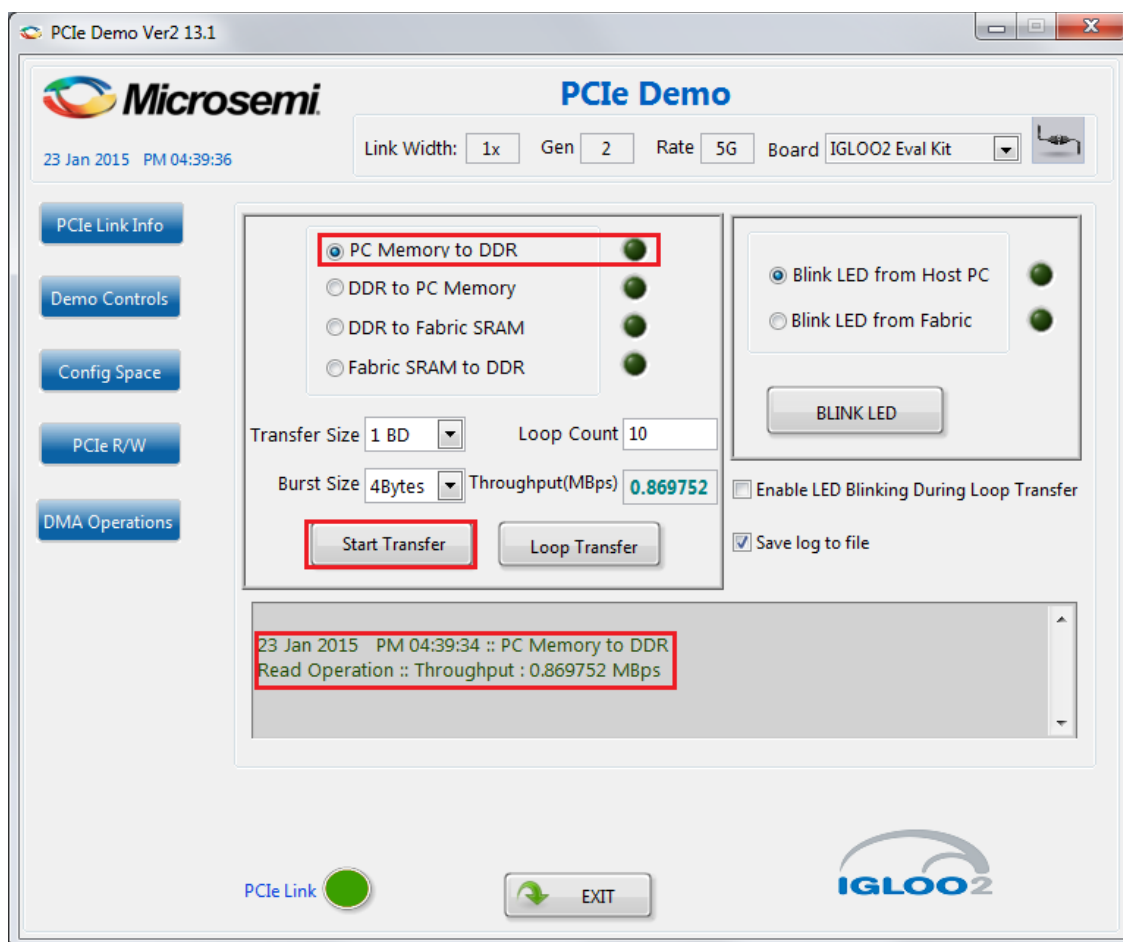
Figure 25 • DMA Transaction - PC Memory to DDR
