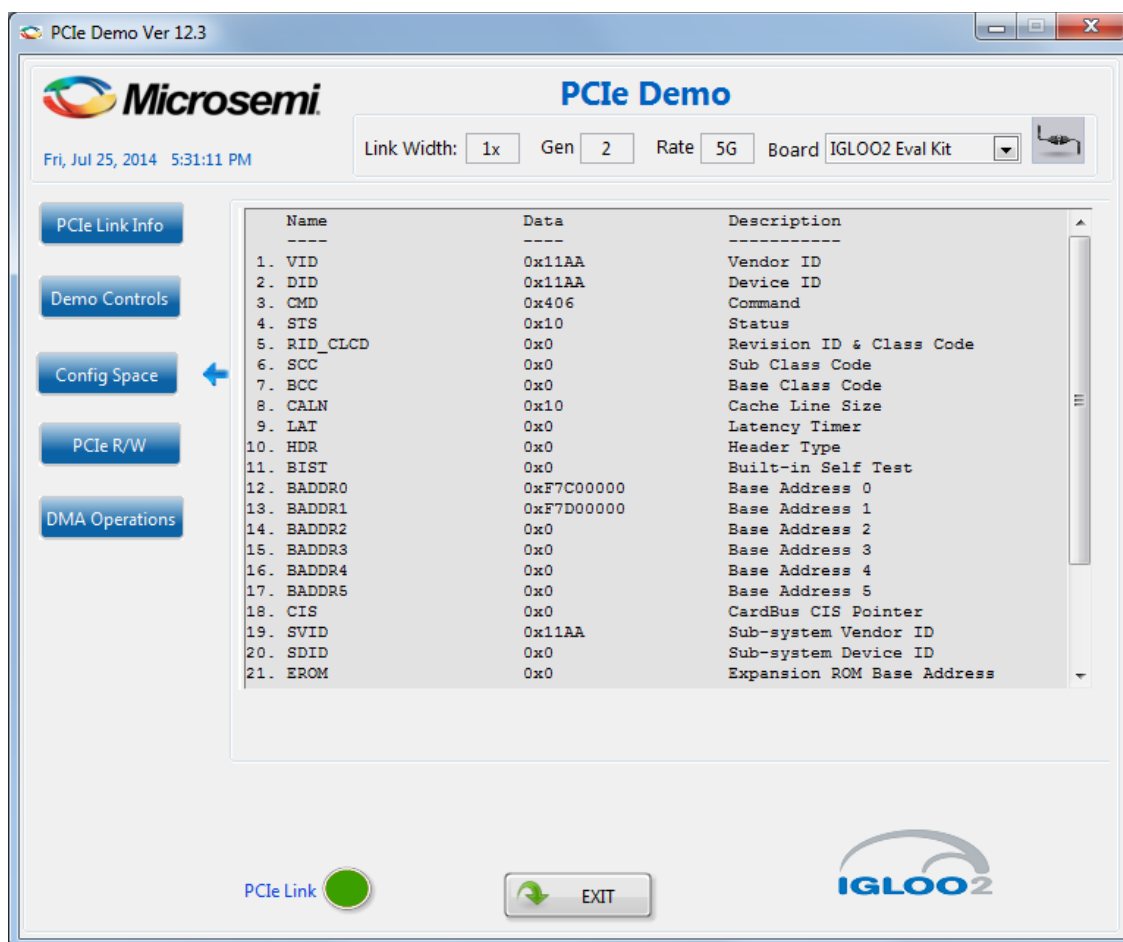
Figure 21 • PCIe Configuration Space
