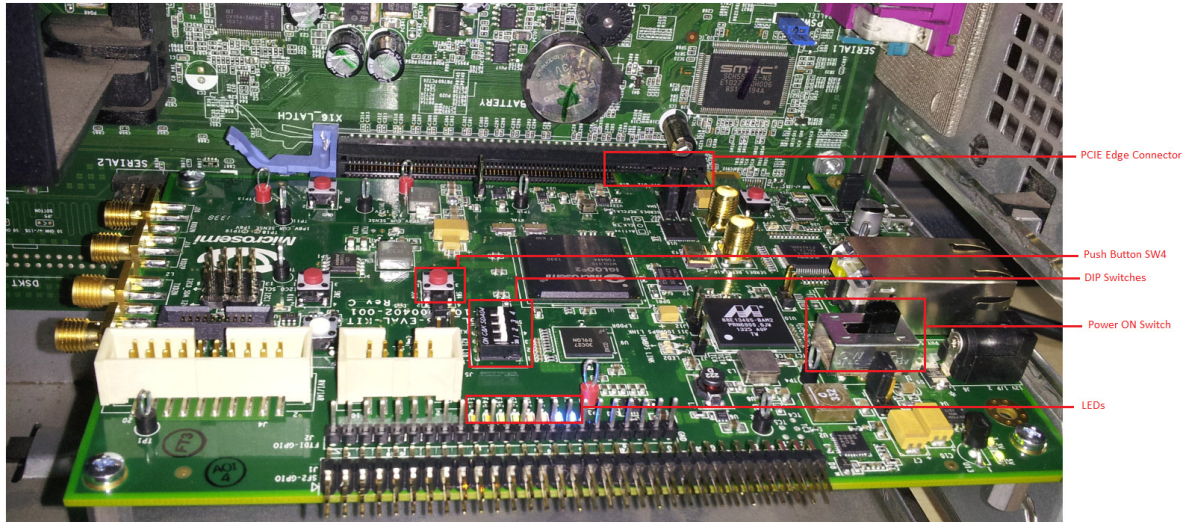
Figure 9 • IGLOO2 Evaluation Kit Setup
