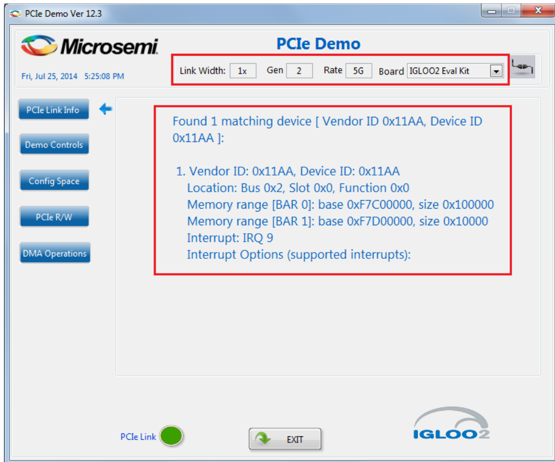
Figure 18 • PCIe Device Information
