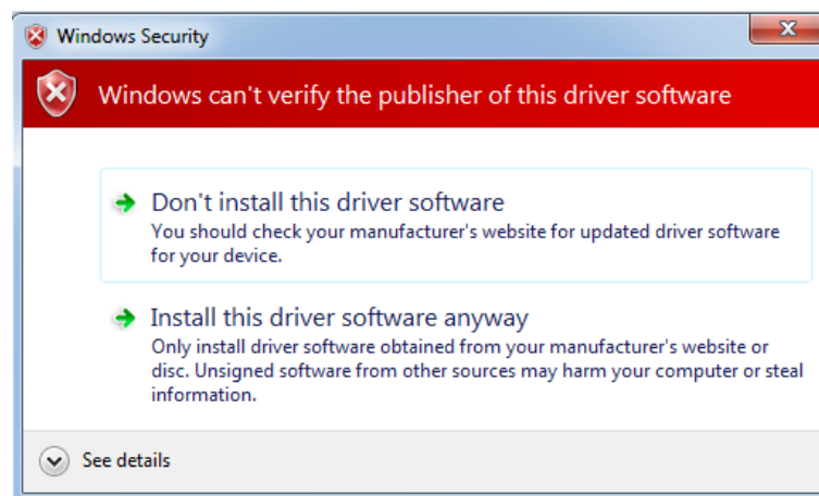
Figure 13 • Windows Security
