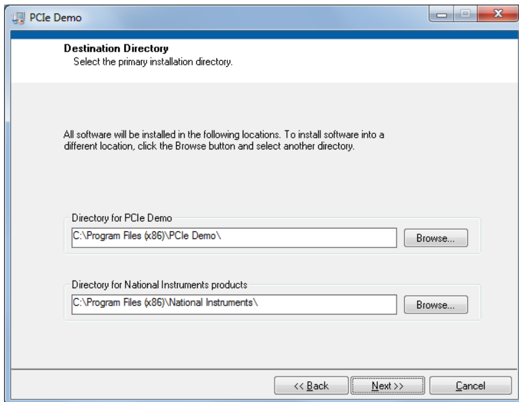
Figure 14 • GUI Installation
