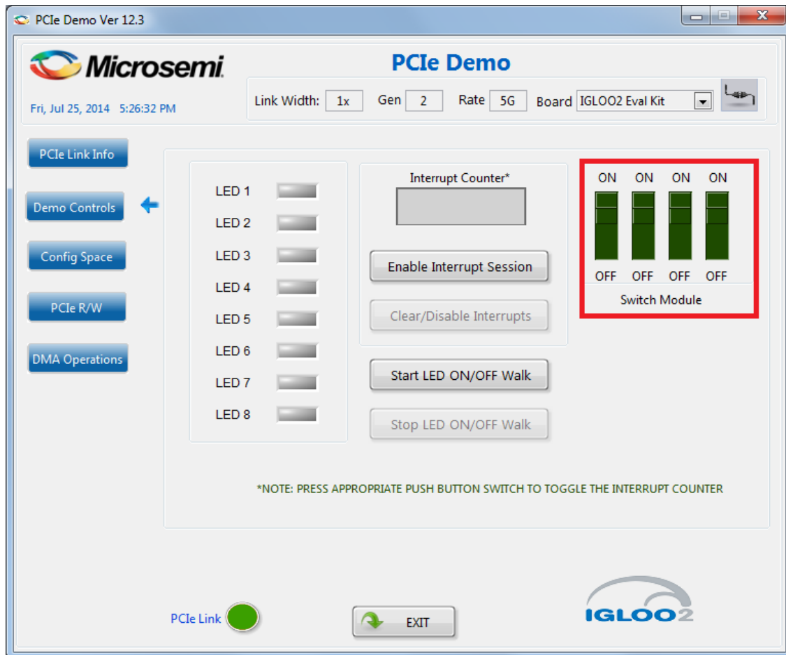
Figure 19 • Demo Controls
