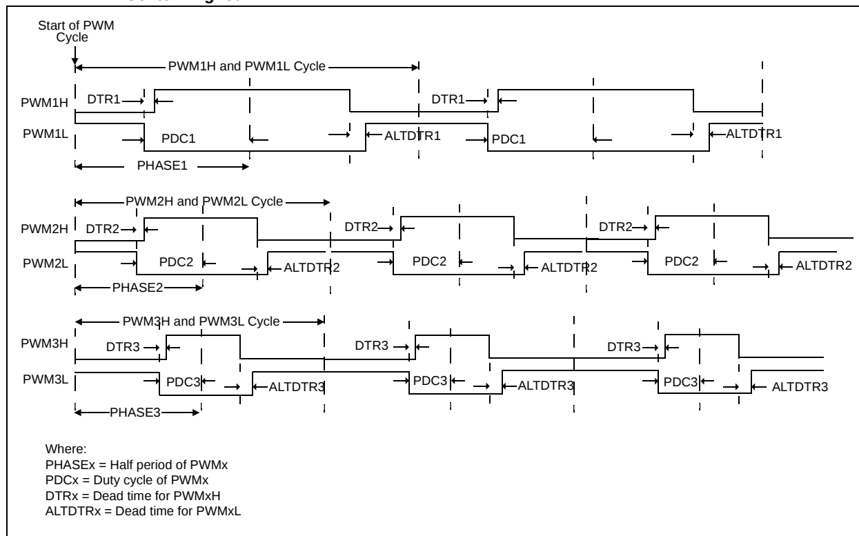
Figure 44-10: Complementary PWM Mode – Independent Duty Cycles and Periods, No Phase-Shifting, Center-Aligned
