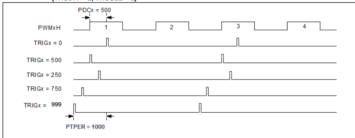
Figure 44-37: Trigger Signal in Relation to PWM Output in Center-Aligned Mode (TRGDIV = 1, TRGSEL = 1)
