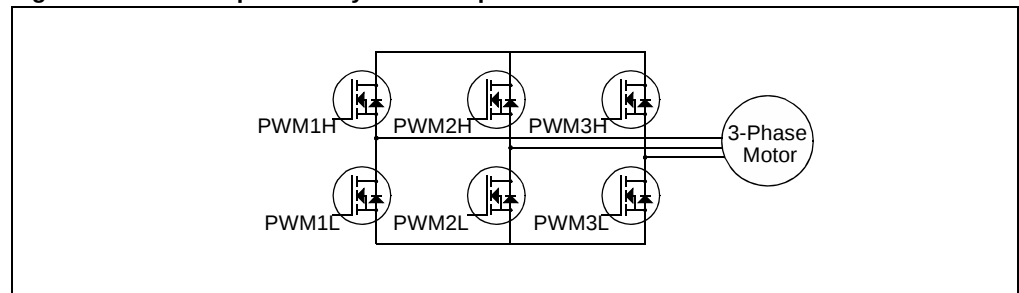
Figure 44-58: Complementary PWM Output Mode for Motor Control
