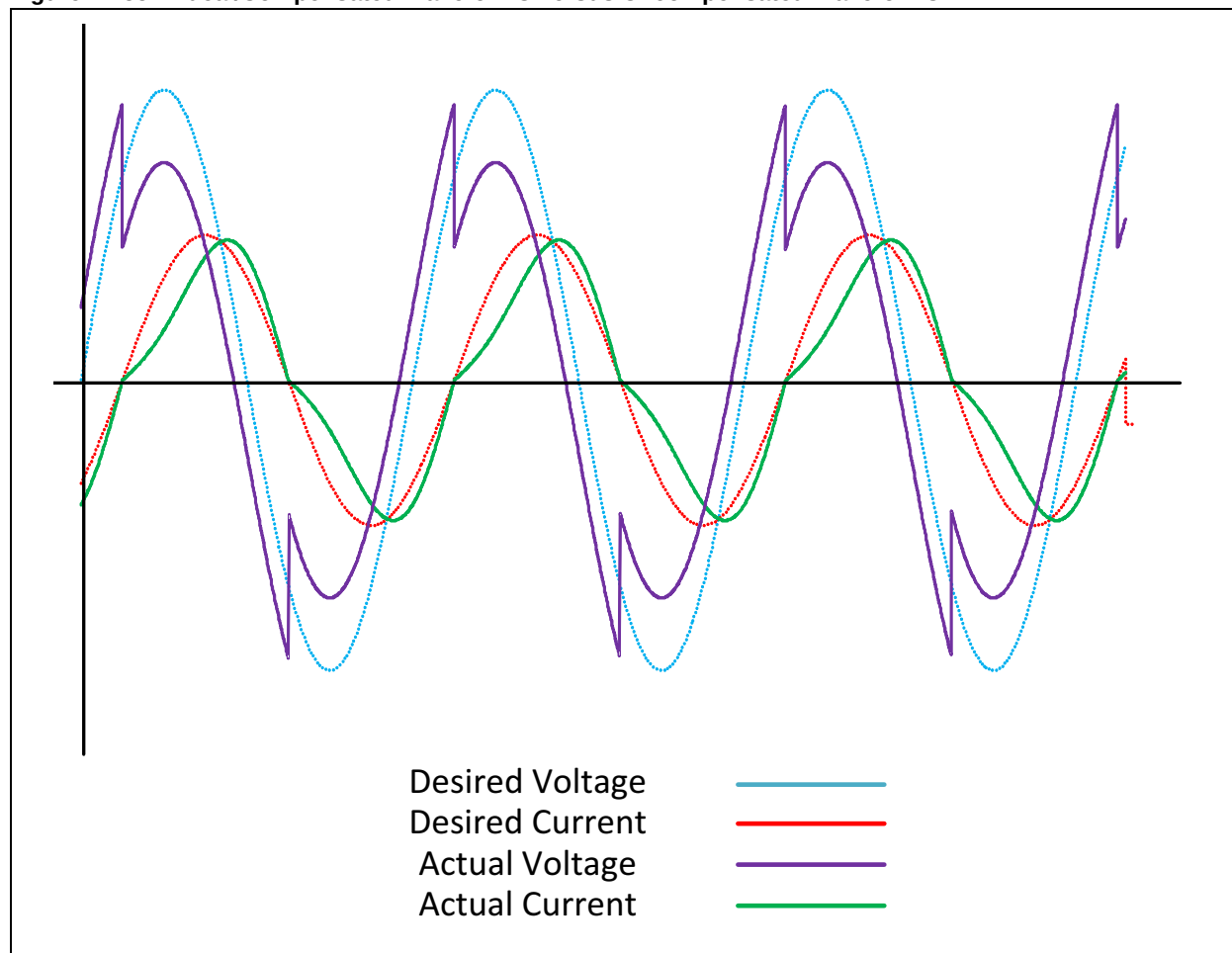
Figure 44-55: Ideal/Compensated Waveforms Versus Uncompensated Waveforms
