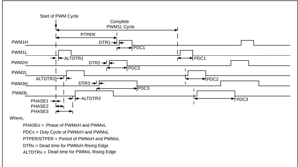
Figure 44-5: Push-Pull PWM Mode – Independent Duty Cycle and Phase, Fixed Period, Edge-Aligned
