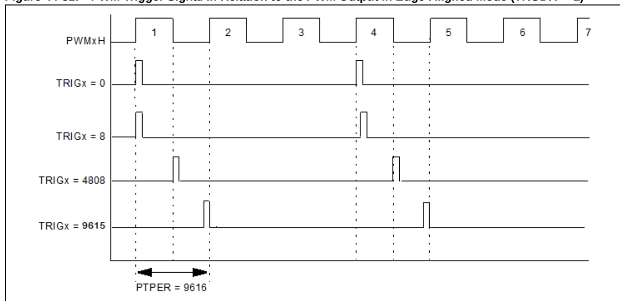
Figure 44-31: PWM Trigger Signal in Relation to the PWM Output in Edge-Aligned Mode (TRGDIV = 2)
