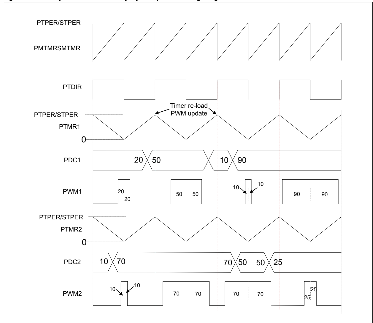
Figure 44-25: Symmetric Mode Duty Cycle Update Timing Diagram
