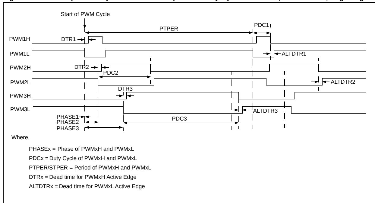
Figure 44-8: Complementary PWM Mode – Independent Duty Cycle and Phase, Fixed Period, Edge-Aligned
