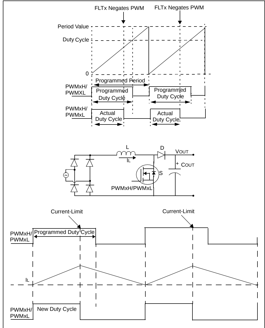
Figure 44-68: Current-Limit PWM
