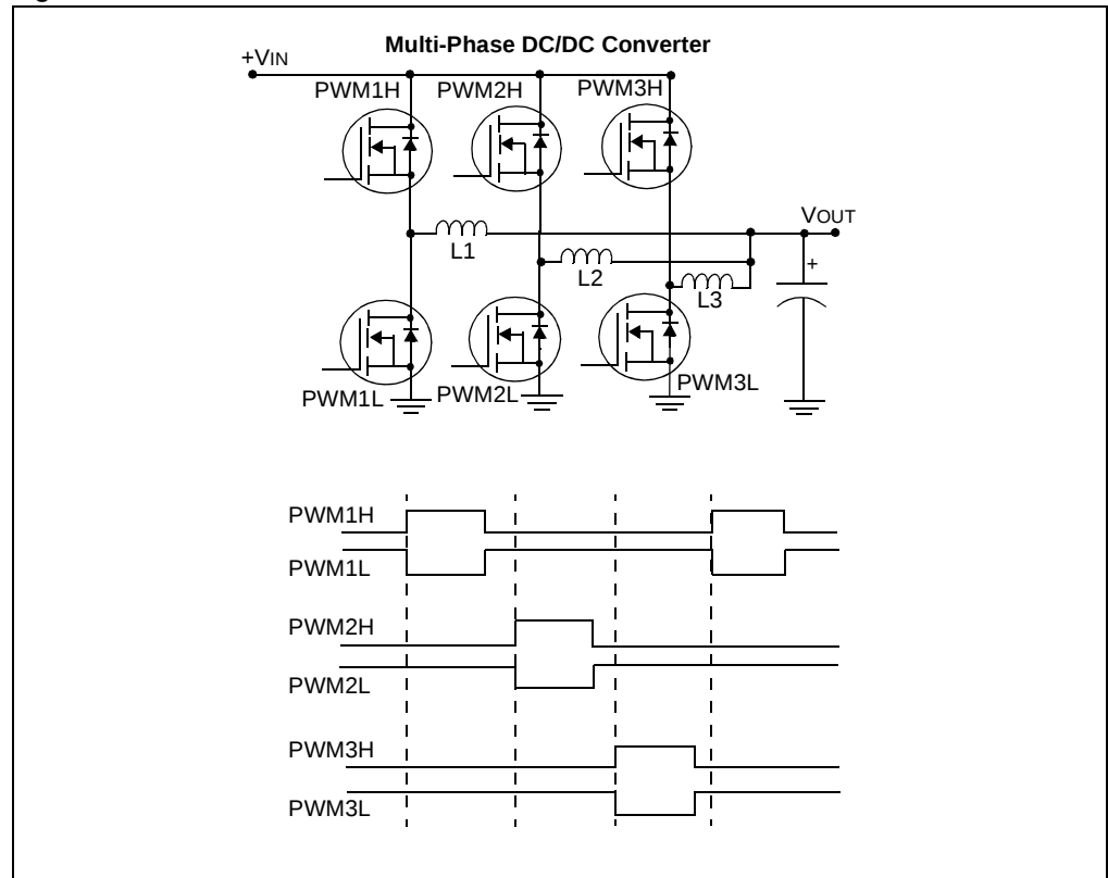
Figure 44-60: Multi-Phase PWM
