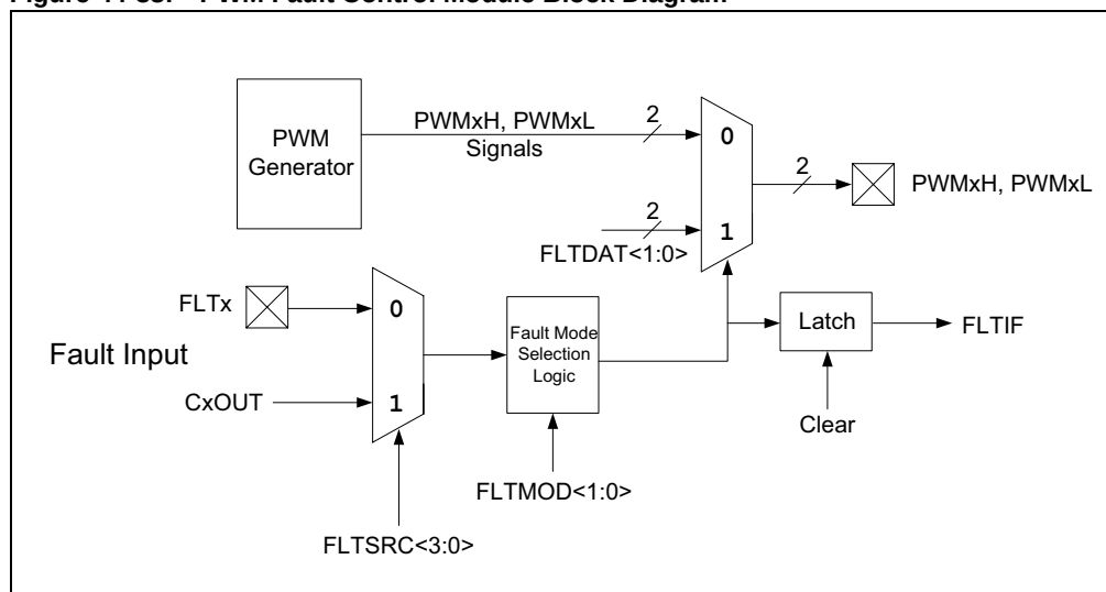
Figure 44-38: PWM Fault Control Module Block Diagram
