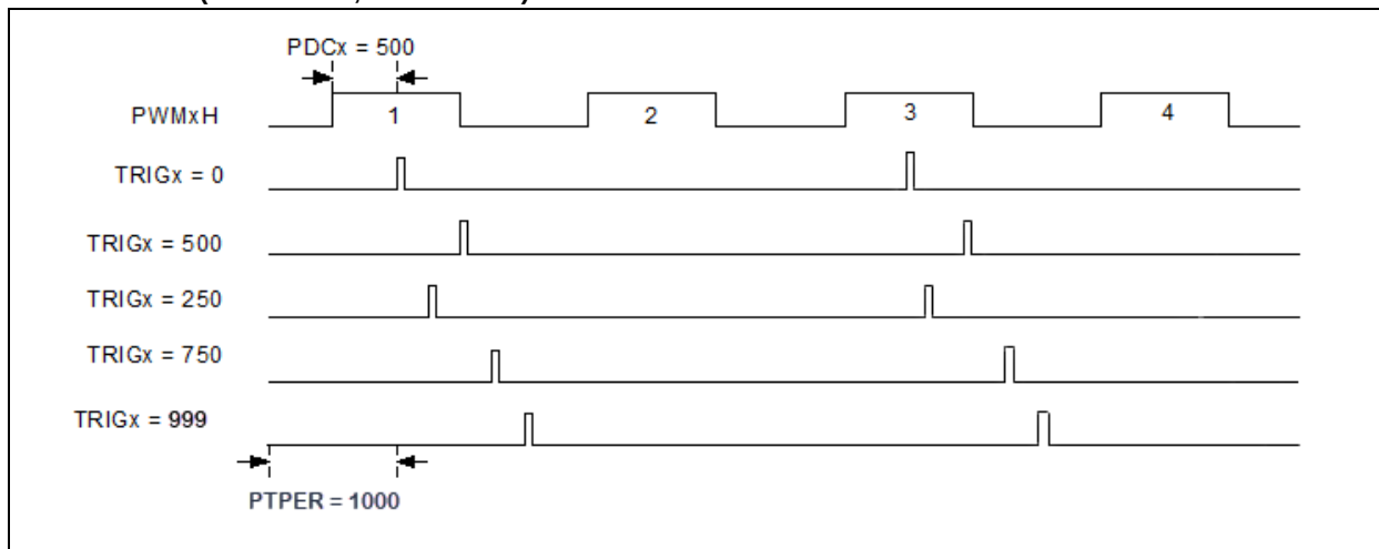
Figure 44-36: Trigger Signal in Relation to PWM Output in Center-Aligned Mode (TRGDIV = 1, TRGSEL = 2)
