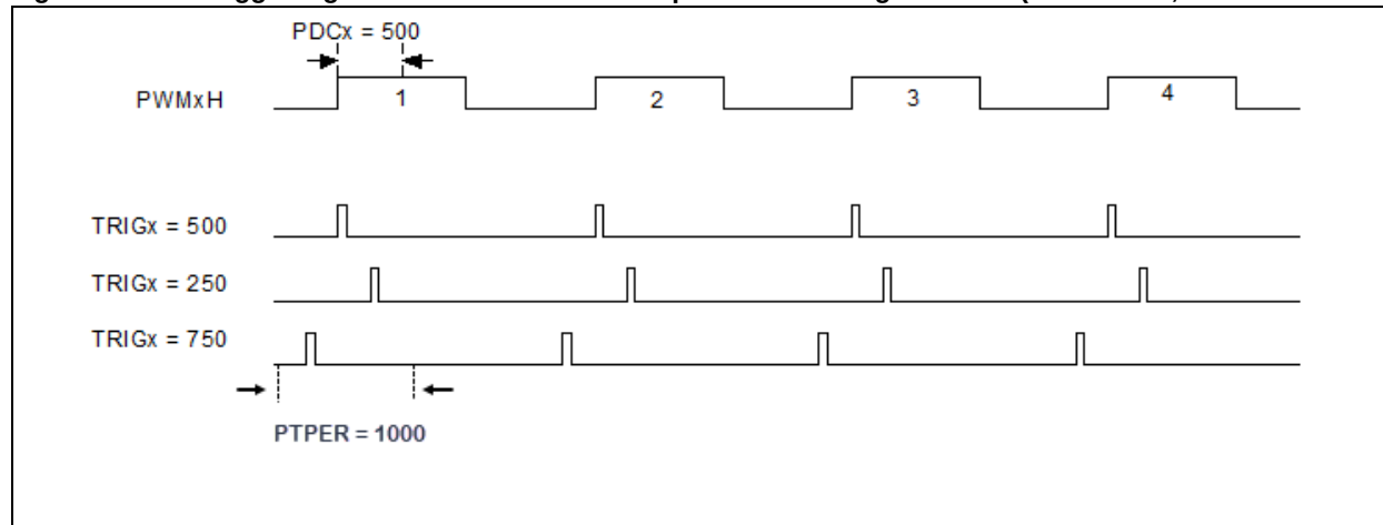
Figure 44-33: Trigger Signal in Relation to PWM Output in Center-Aligned Mode (TRGDIV = 1, TRGSEL = 0 or 3)
