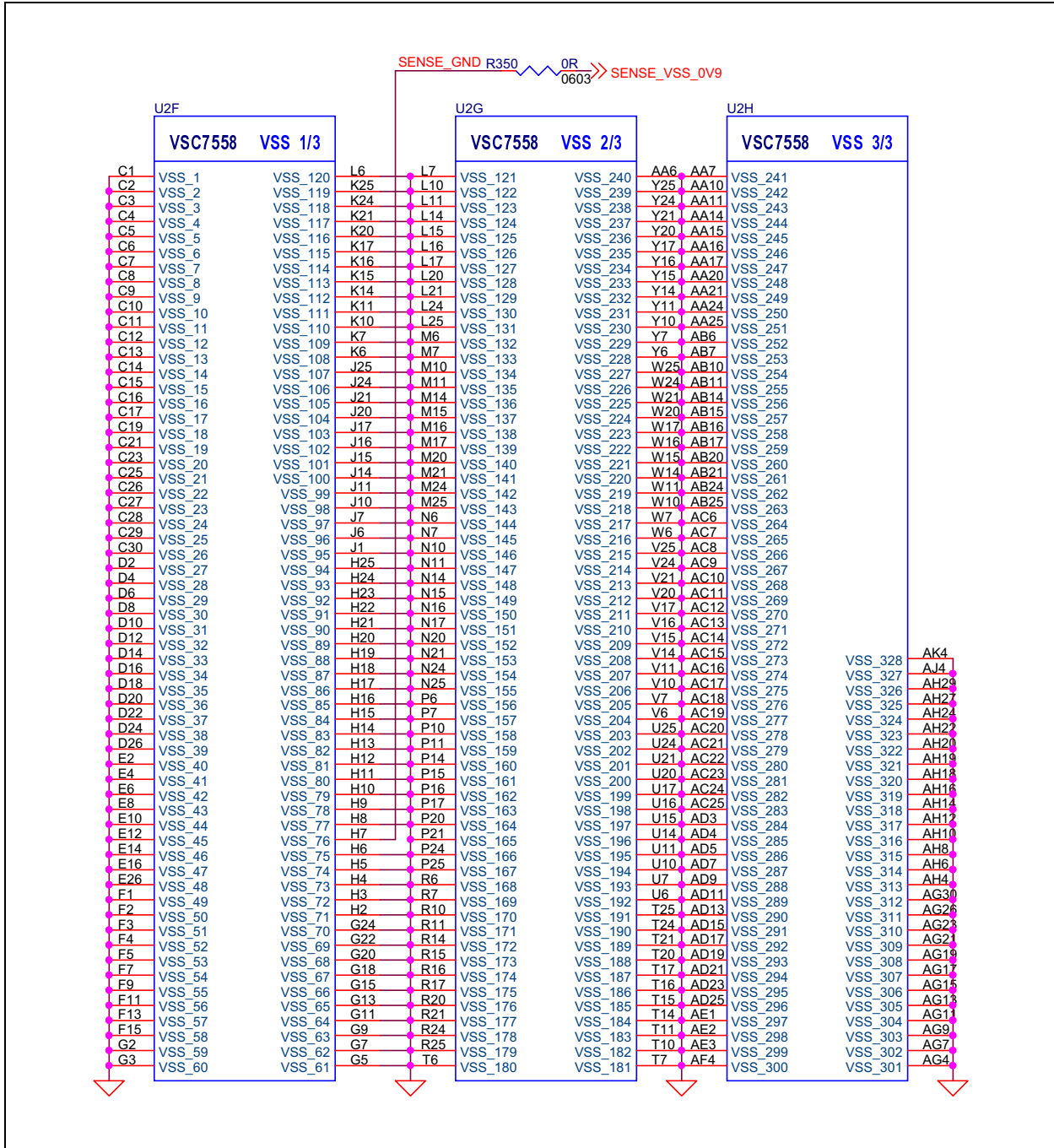
FIGURE 3-2: GROUND PINS
