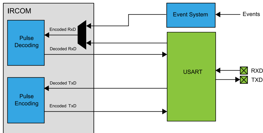
Figure 27-13. Block Diagram
