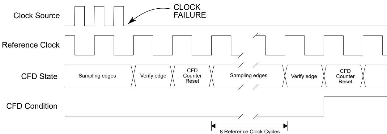
Figure 12-5. Clock Failure Detection (CFD) Timing Diagram
