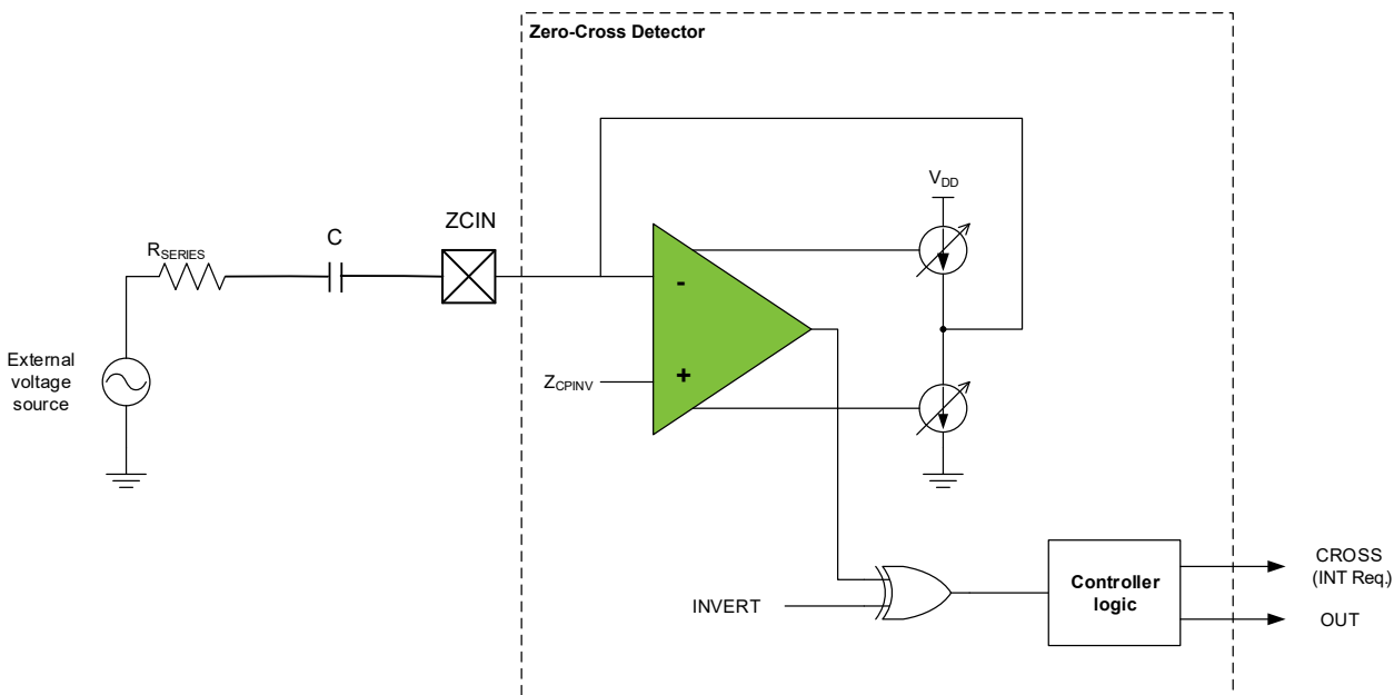
Figure 35-7. AC Coupling the ZCD
