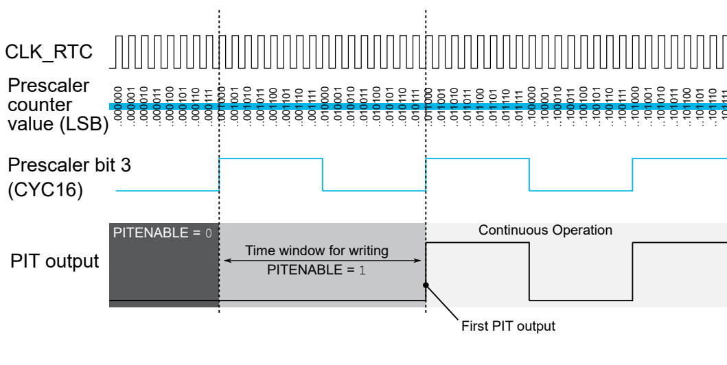
Figure 26-2. Timing Between PIT Enable and First Interrupt
