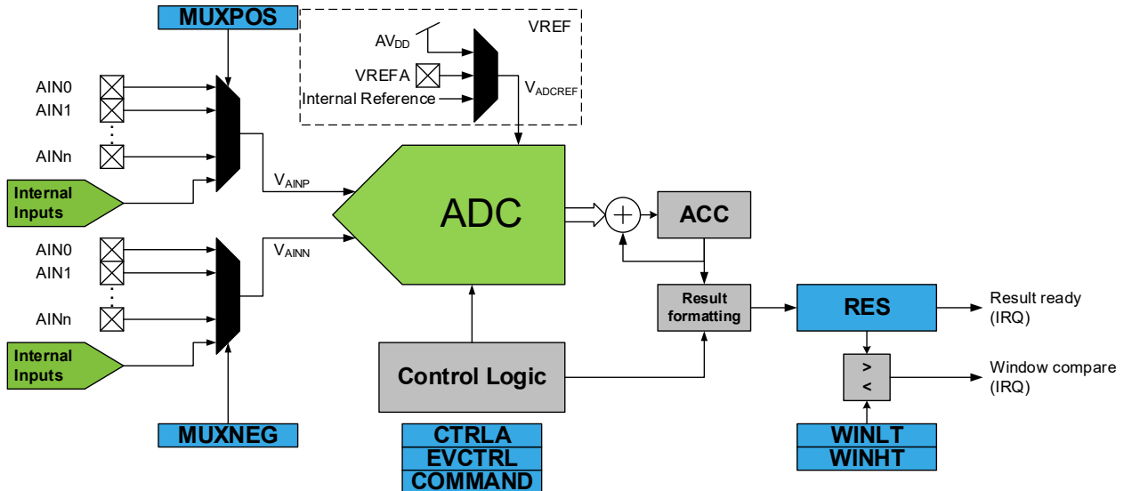
Figure 33-1. Block Diagram
