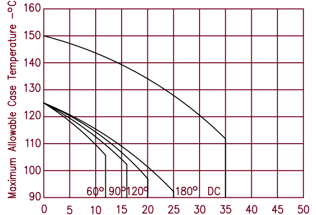
Figure 5 Forward Current Derating — Reverse Polarity
