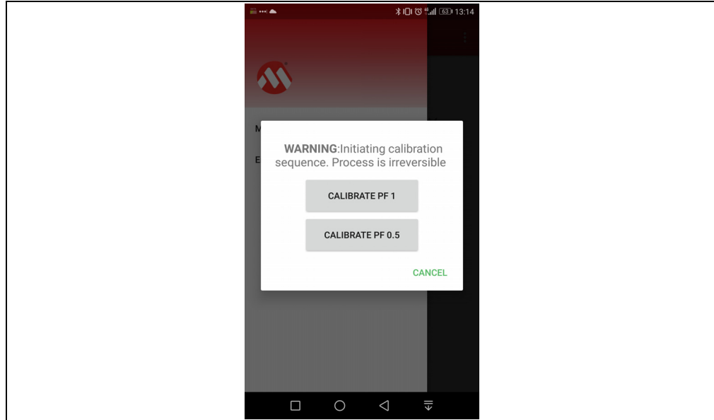
FIGURE 4-6: Calibration Menu.
