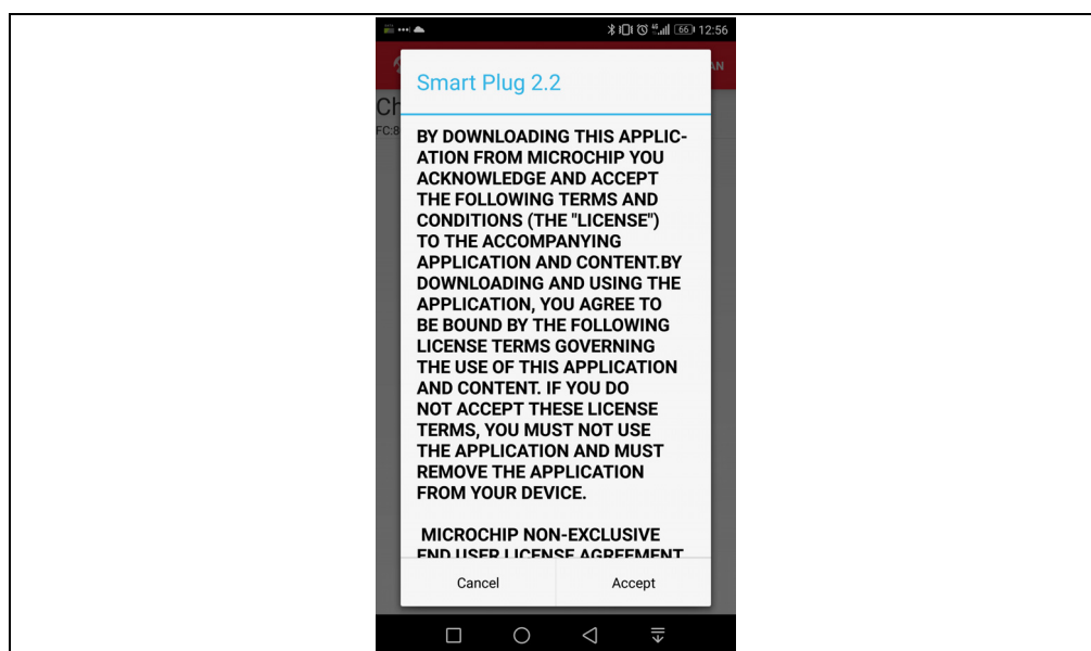
FIGURE 4-1: License Agreement.
