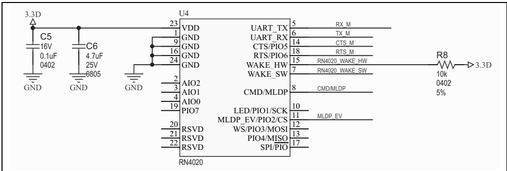
FIGURE 1-10: RN4020.
