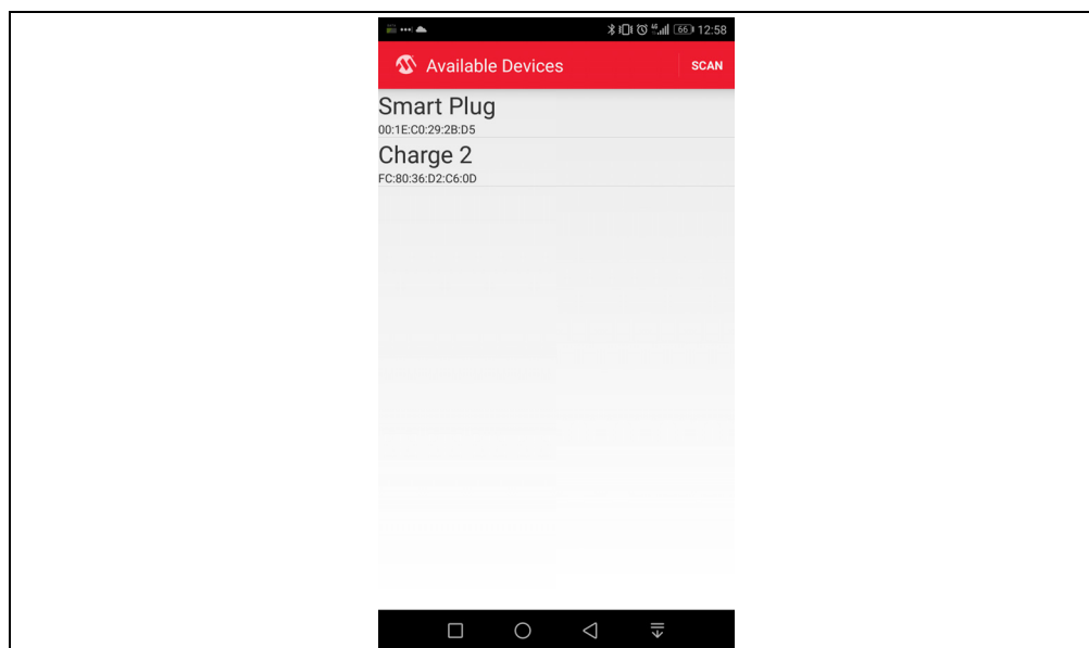
FIGURE 4-2: Device List.
