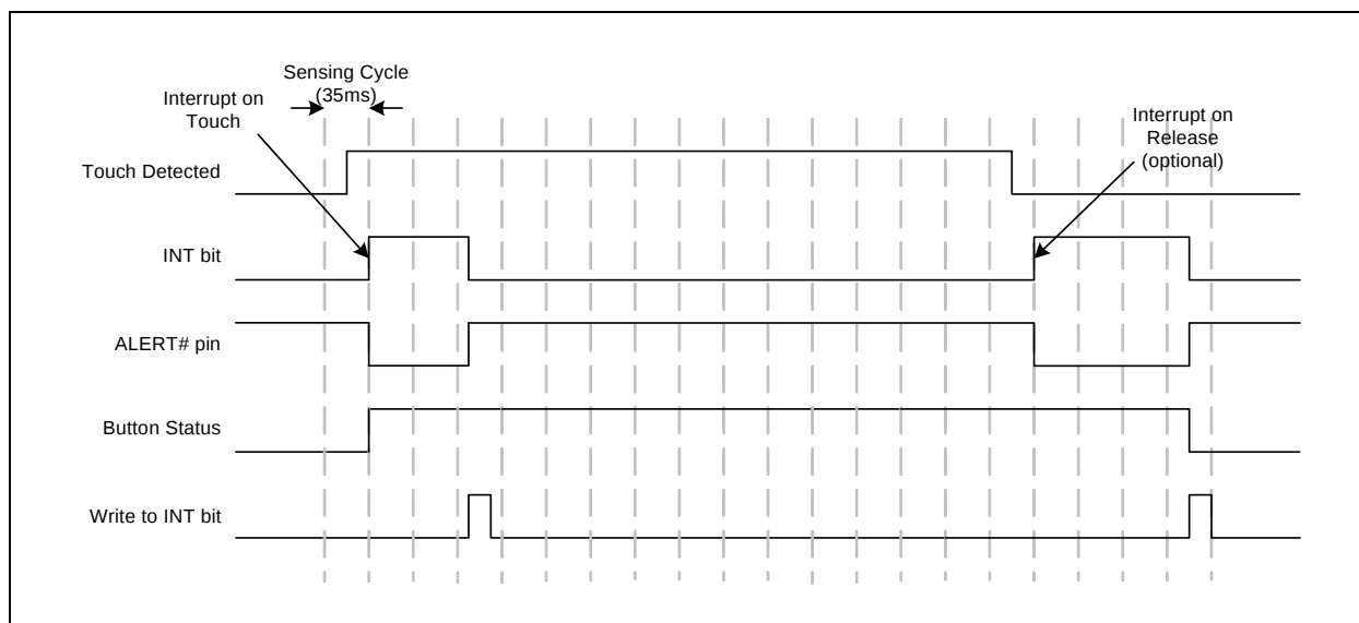
FIGURE 4-5: SENSOR INTERRUPT BEHAVIOR - NO REPEAT RATE ENABLED
