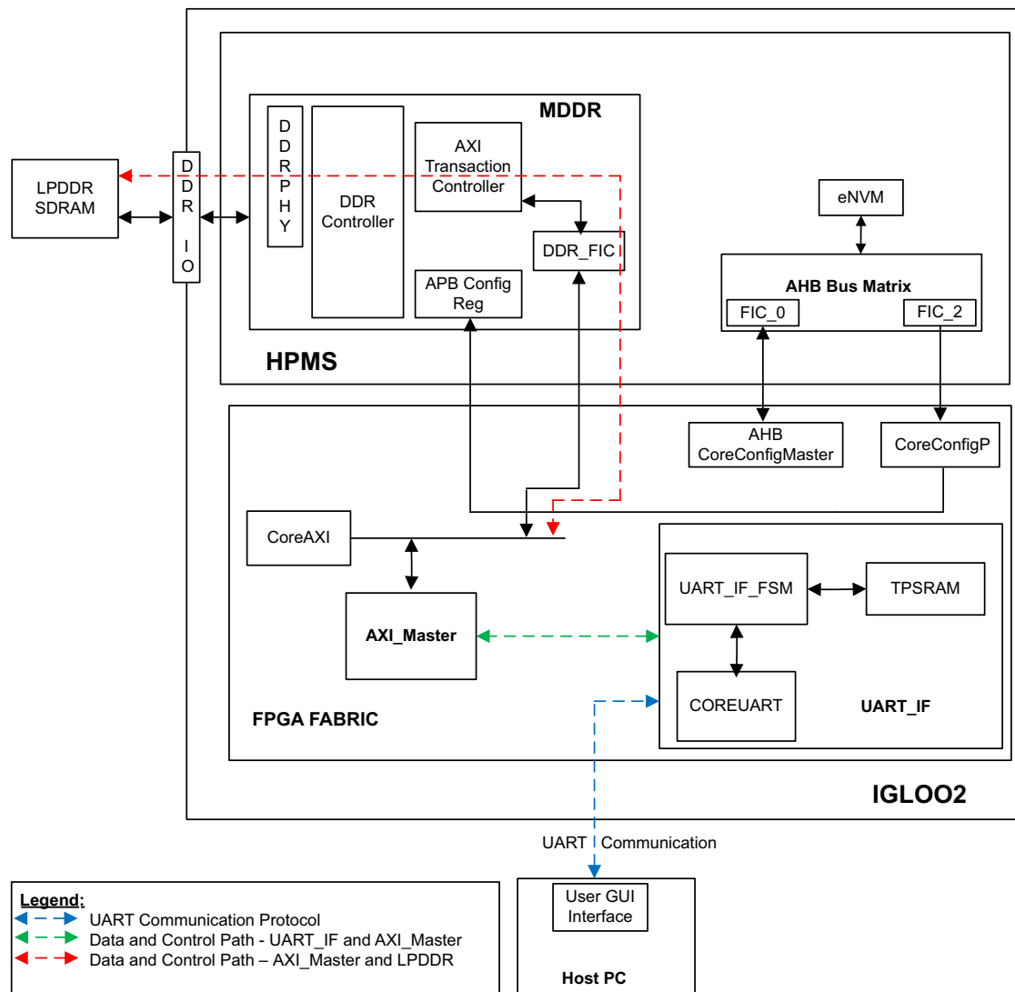
Figure 3 • MDDR Demo Design Block Diagram - IGLOO2
