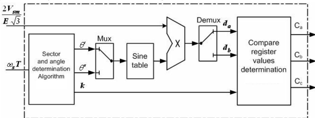
Figure 3-7. Space Vector PWM data flow diagram
