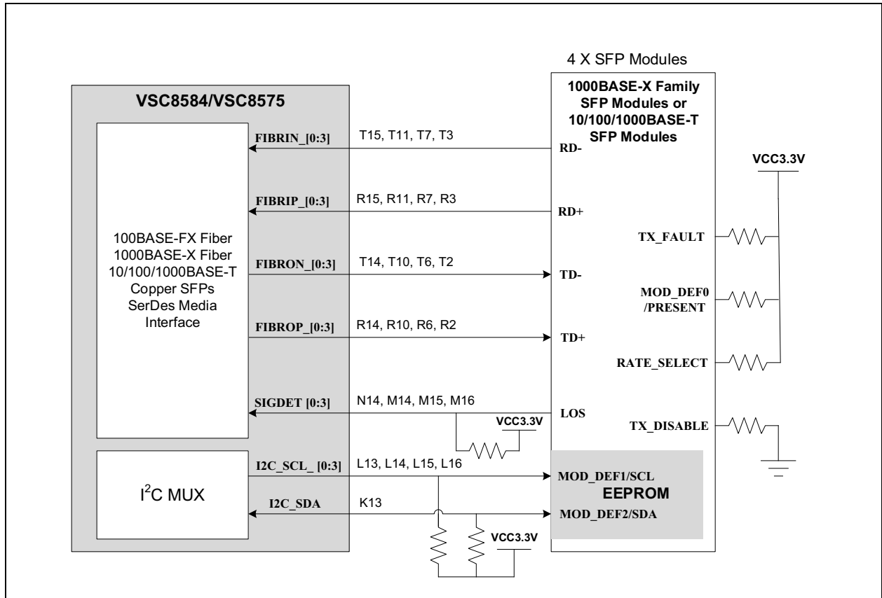
FIGURE 5-1: SERDES MEDIA INTERFACE TO 1000BASE-X FAMILY FIBER SFP OR 10/100/1000BASE-T COPPER SFP REFERENCE CONNECTION
