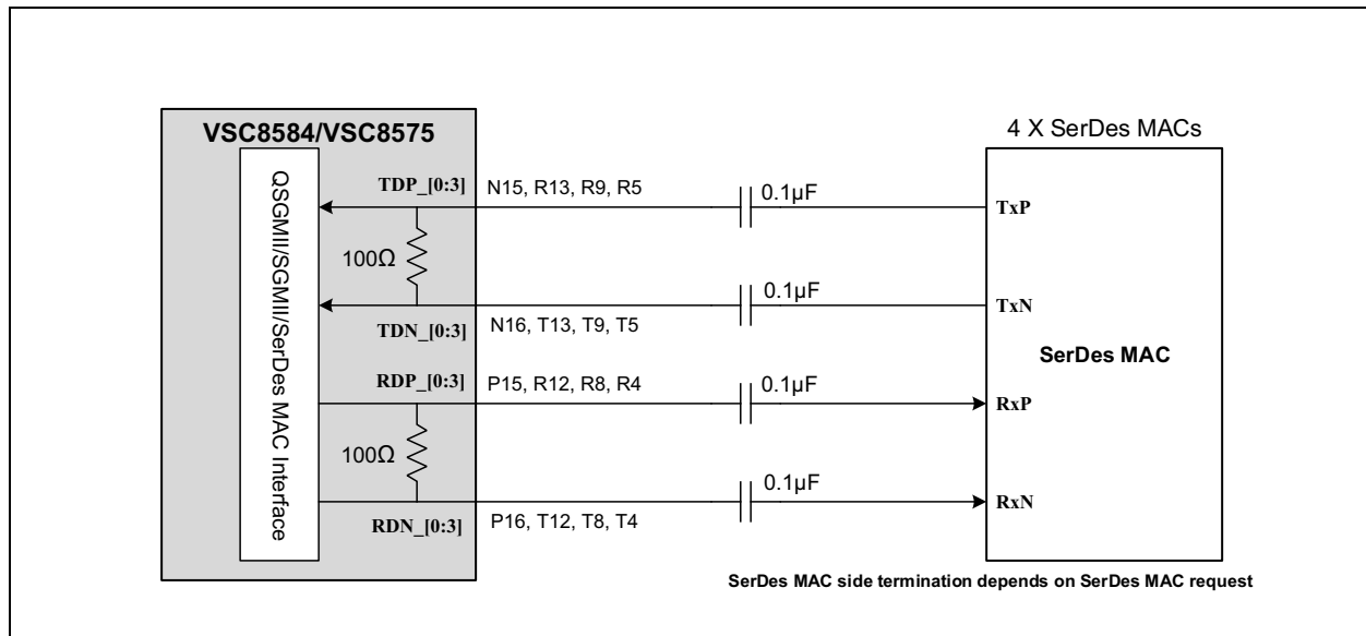
FIGURE 6-3: SERDES MAC INTERFACE CONNECTIONS
