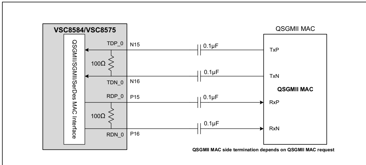
FIGURE 6-1: QSGMII MAC INTERFACE CONNECTIONS
