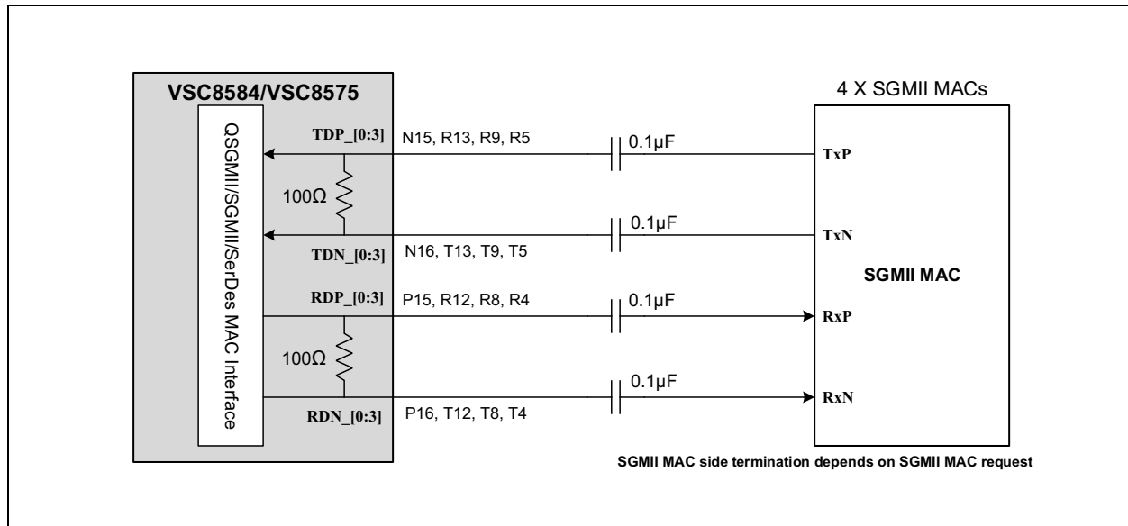
FIGURE 6-2: SGMII MAC INTERFACE CONNECTIONS
