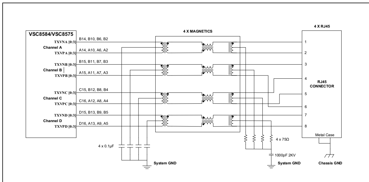
FIGURE 4-1: SOLUTION #1 FOR 10/100/1000 MBPS CHANNEL CONNECTIONS
