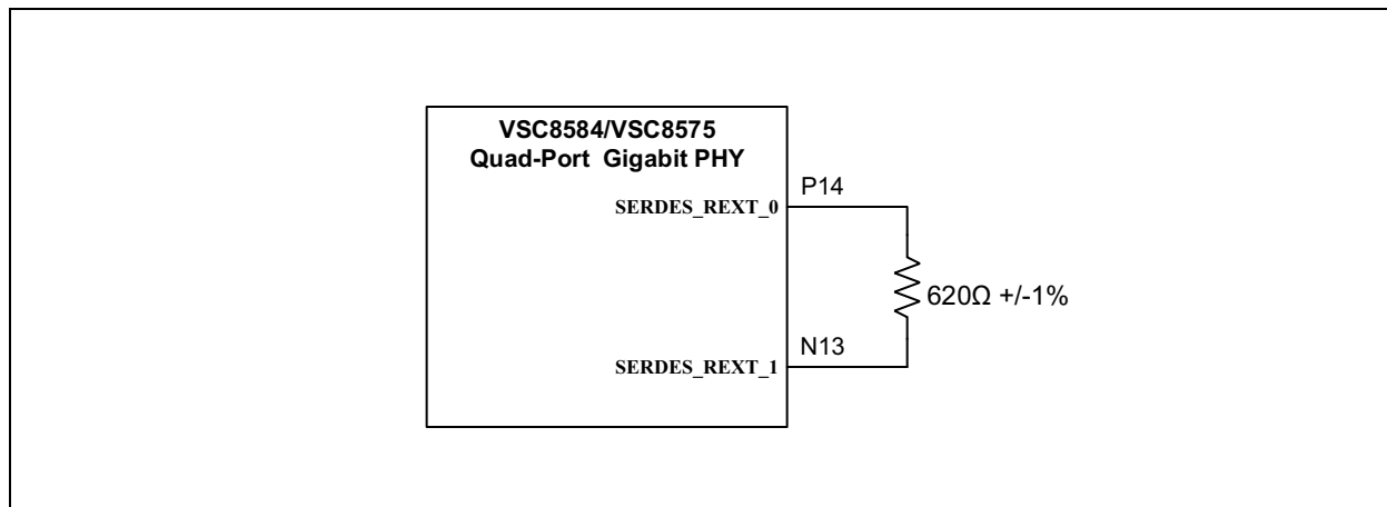
FIGURE 10-1: SERDES BIAS RESISTOR
