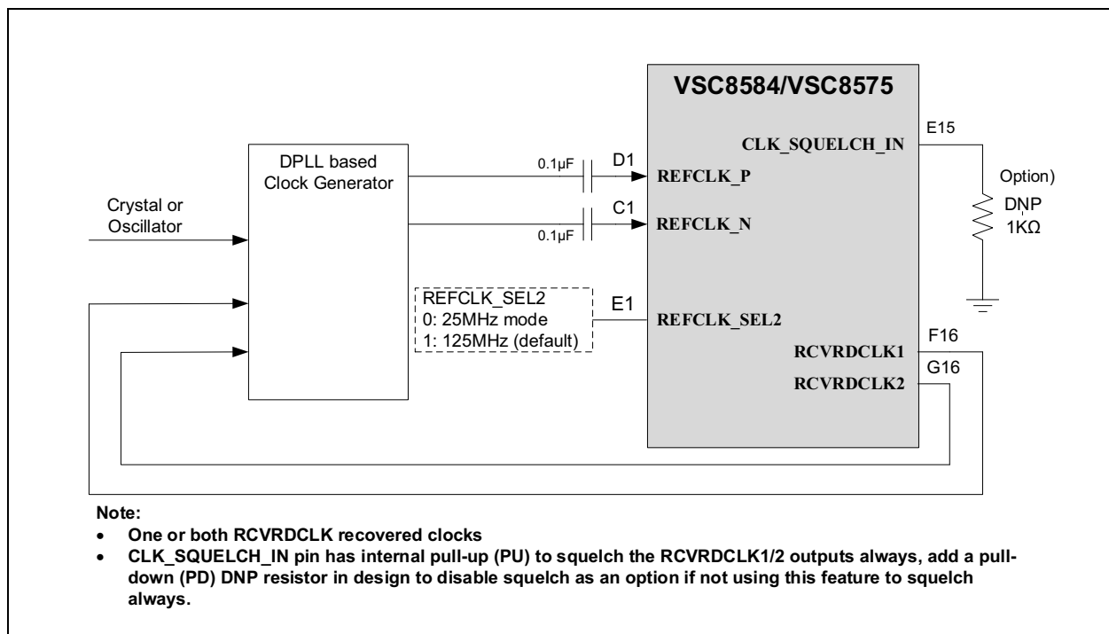
FIGURE 7-3: TYPICAL SYNCHRONOUS ETHERNET CLOCK CONFIGURATION
