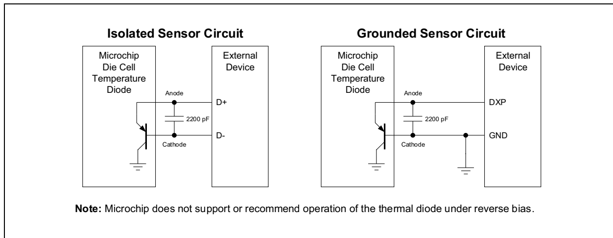
FIGURE 10-3: THERMAL DIODE CONNECTIONS
