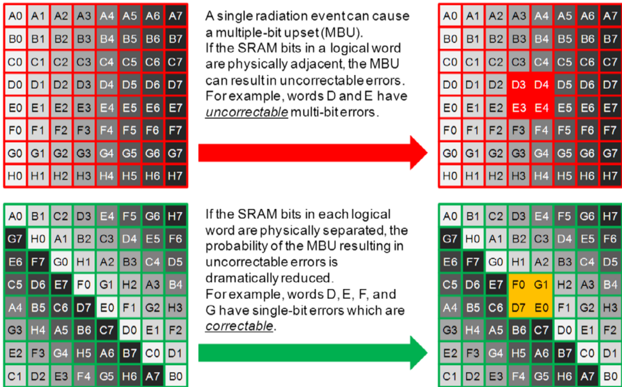
Figure 1: Illustration of Mitigation of Multiple Bit Upsets by Physical Interleaving of Memory Cells
