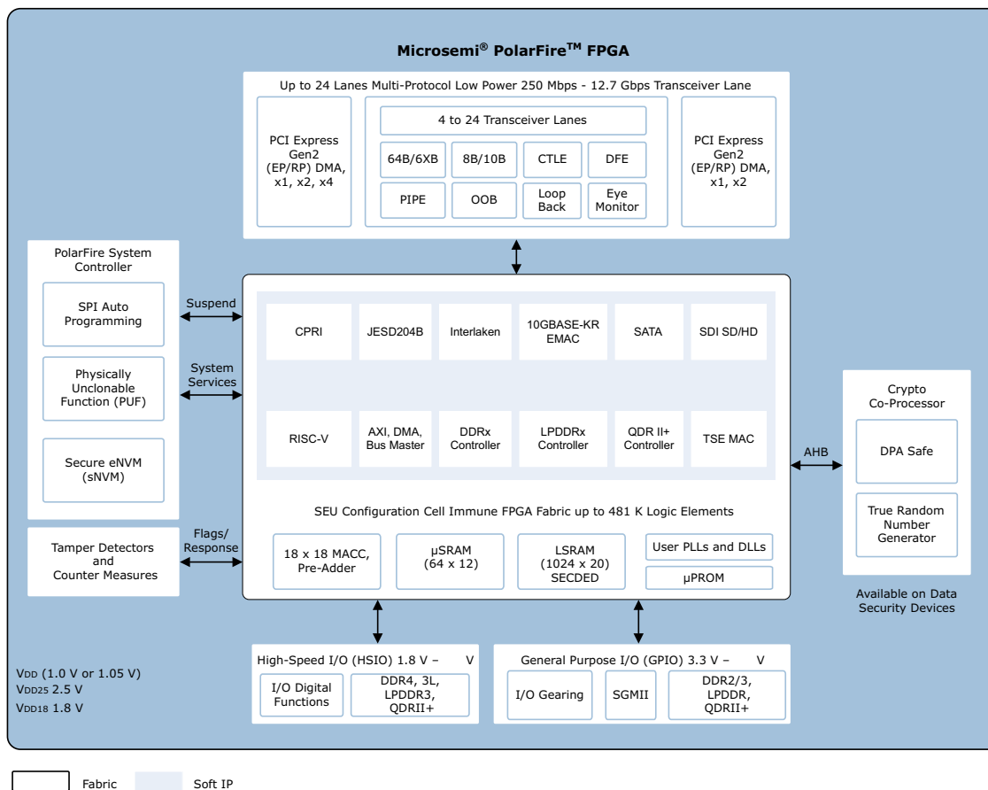
Figure 1 • Device Architecture
