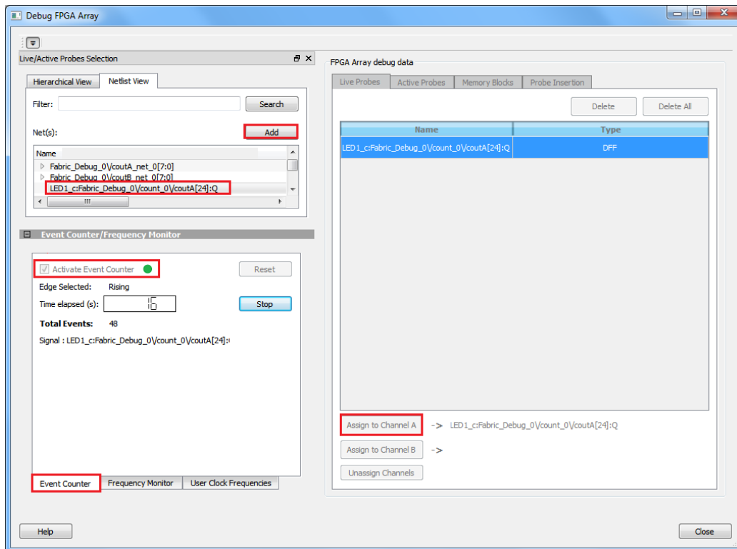
Figure 18 • Event Counter
