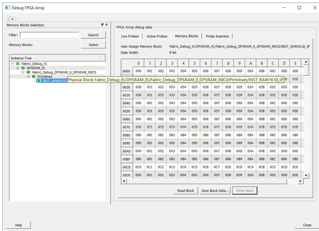
Figure 35 • Displaying Tooltip for Memory Blocks
