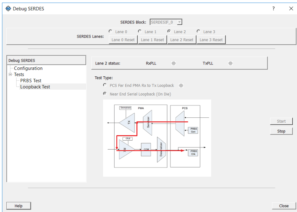
Figure 51 • Loopback Test Feature
