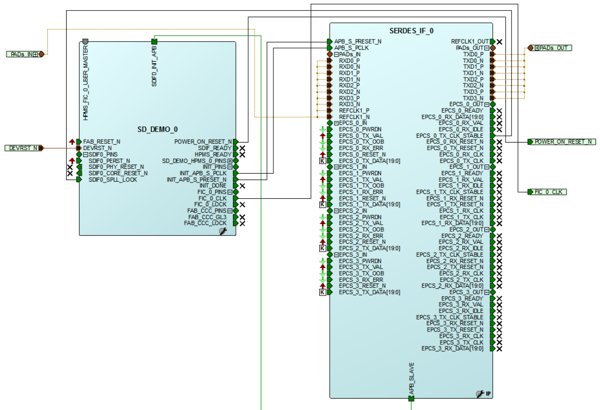
Figure 3 • Fabric_Debug Overall Design Blocks (IGLOO2 Design Block)
