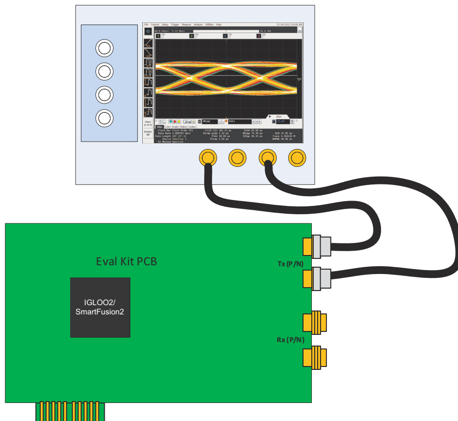
Figure 46 • Connecting Lane 2 to the Test Equipment
