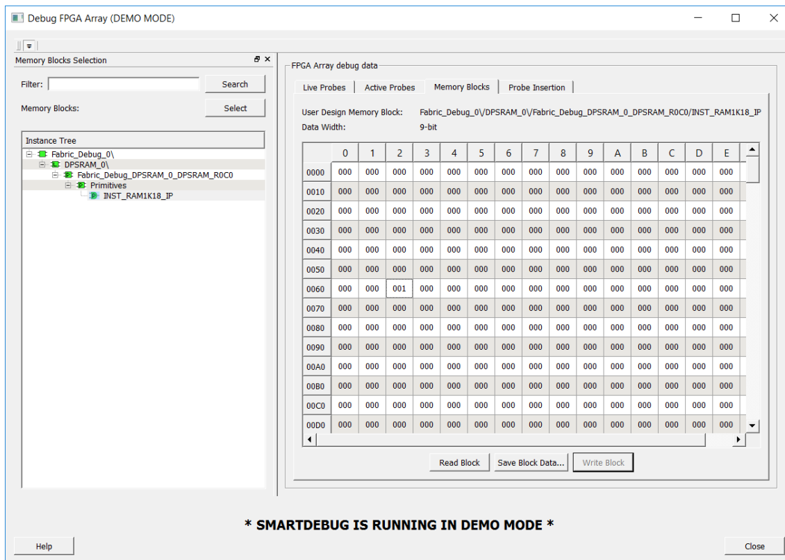
Figure 63 • Memory Blocks in Demo Mode
