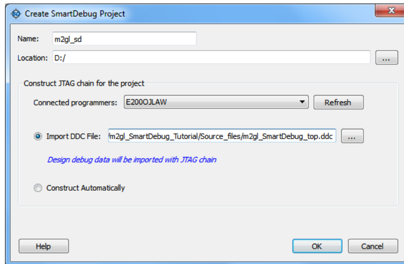
Figure 57 • Create SmartDebug Project
