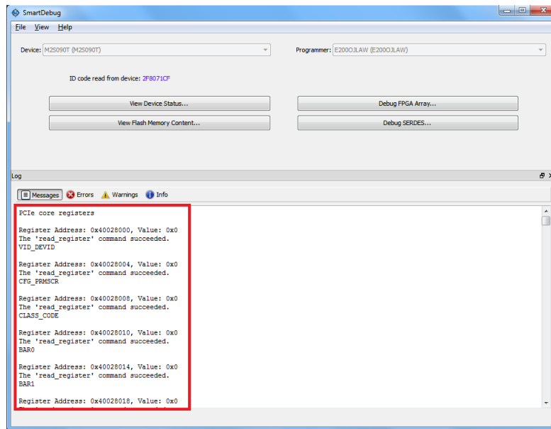
Figure 53 • SerDes Access Log
