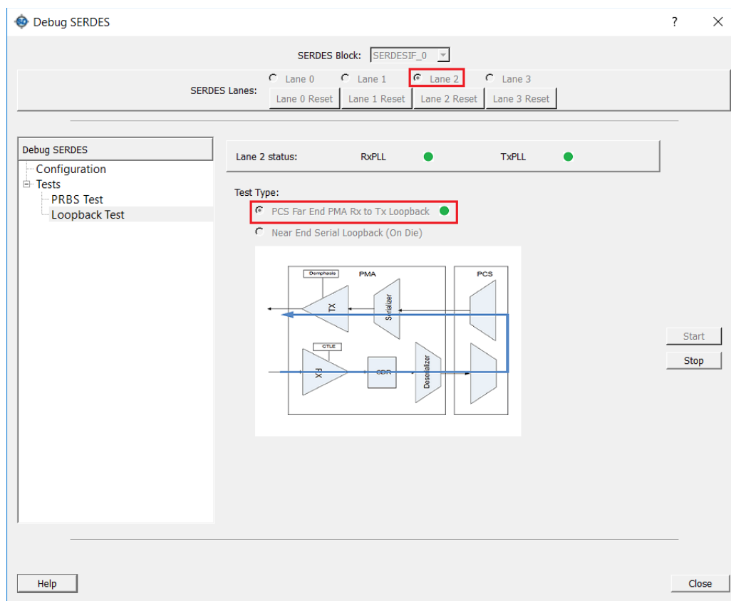
Figure 50 • PCS Far-End Rx to Tx Loopback
