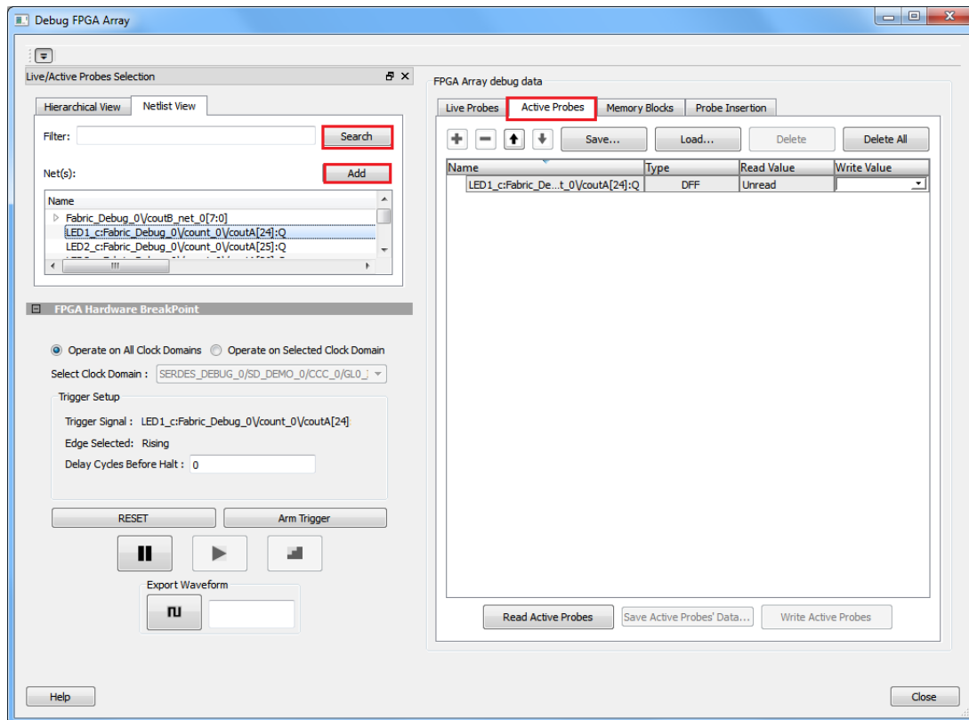
Figure 21 • Selecting Active Probes From the Design
