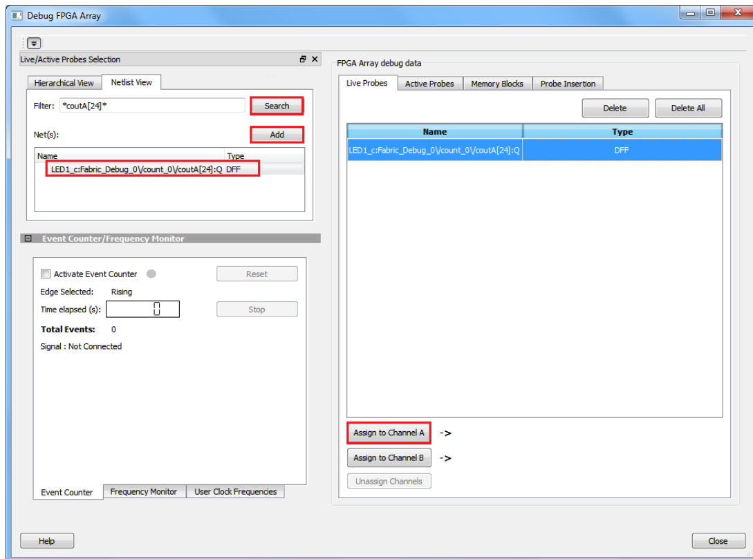
Figure 17 • Live Probes Channels Assignments
