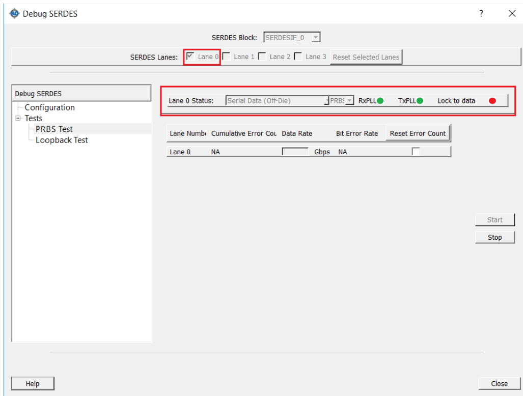
Figure 42 • Sending Serial Tx Data Off-Die—Lane 0
