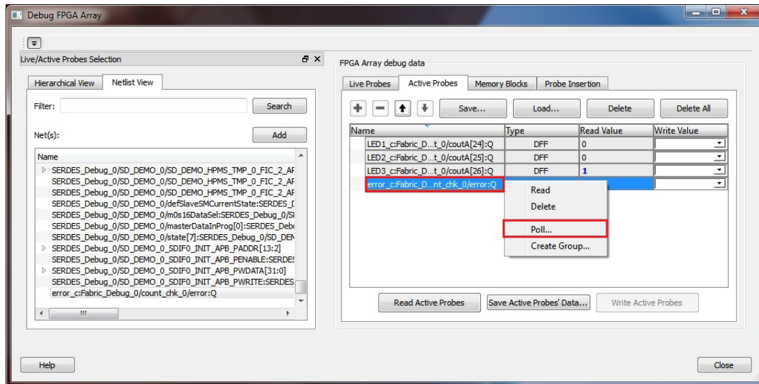
Figure 24 • Pseudo Static Signal Poll
