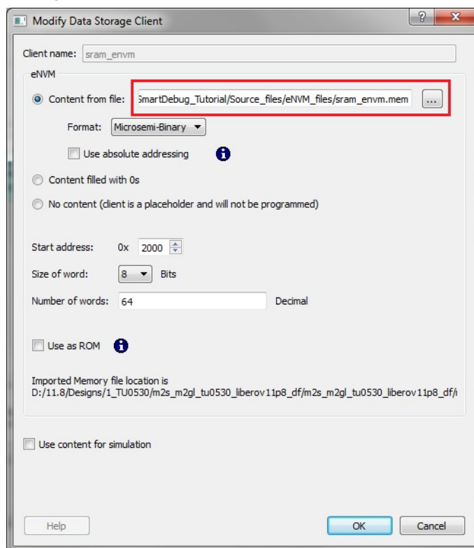
Figure 6 • Modify Data Storage Client Window
