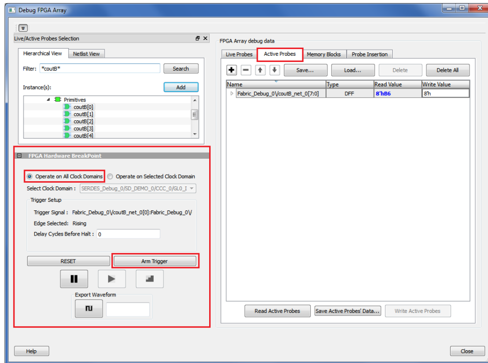
Figure 30 • Select Clock Domain
