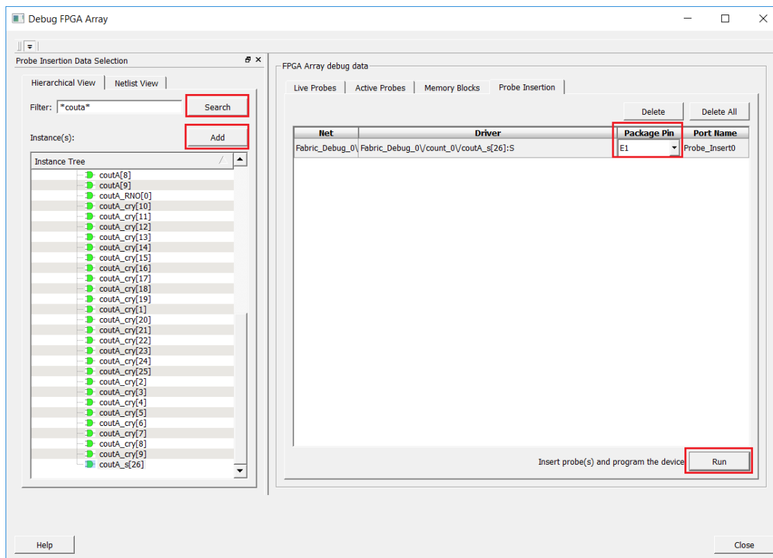
Figure 37 • Assigning Package Pin and Running the Flow
