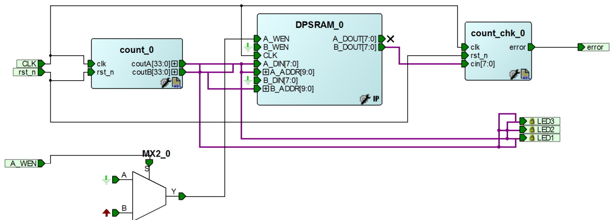
Figure 3 • Fabric_Debug Overall Design Blocks (IGLOO2 Design Block)
