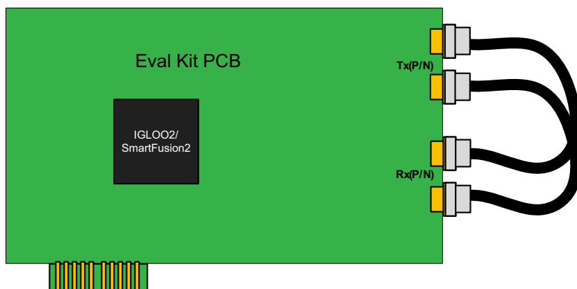
Figure 44 • Evaluation Kit Board with External Coax Loopback Setup
