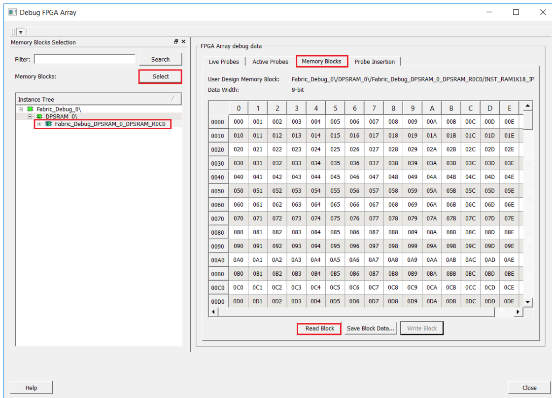
Figure 34 • DPSRAM_0 Contents
