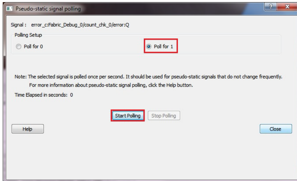
Figure 25 • Polling Setup Selection
