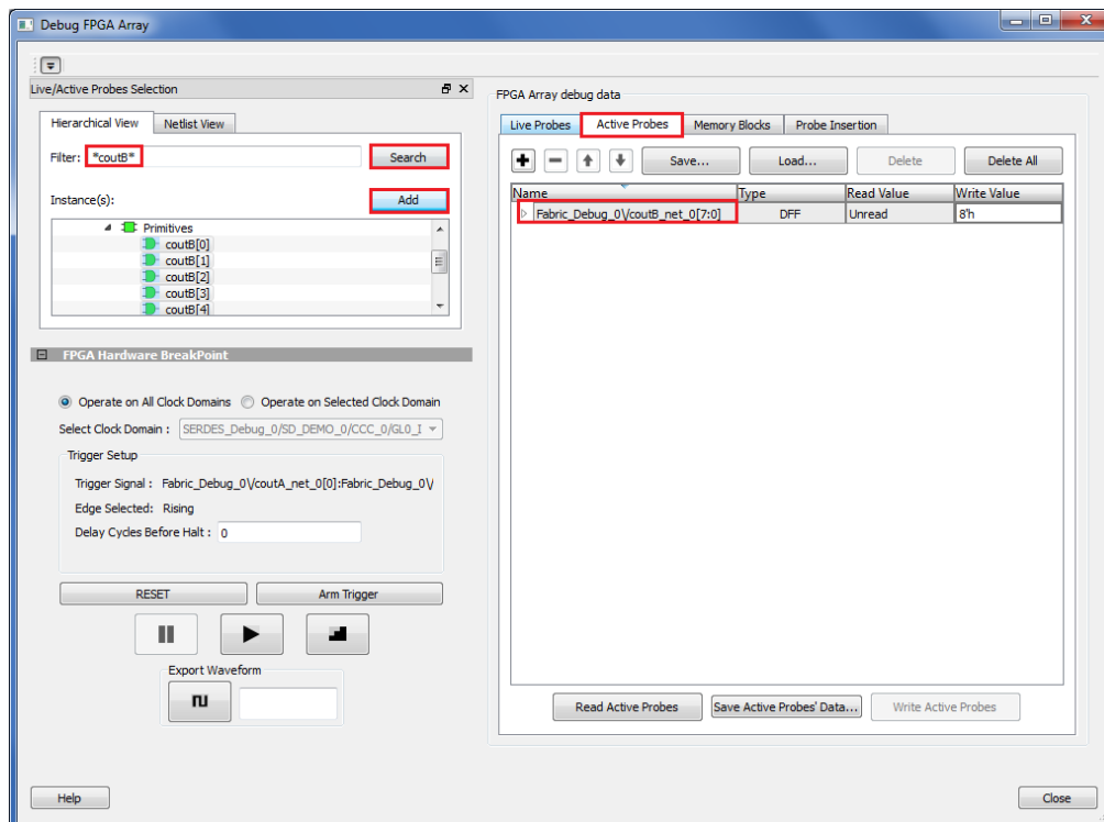
Figure 29 • Add couB[0]–coutB[7] to Active Probes
