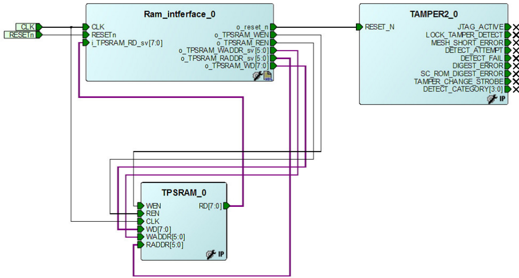
Figure 45 • Dev_Restart_after_IAP_blk SmartDesign
