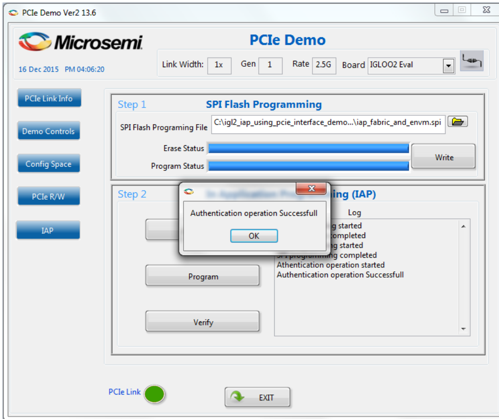
Figure 24 • IAP Authentication Success Message in PCIe Demo GUI
