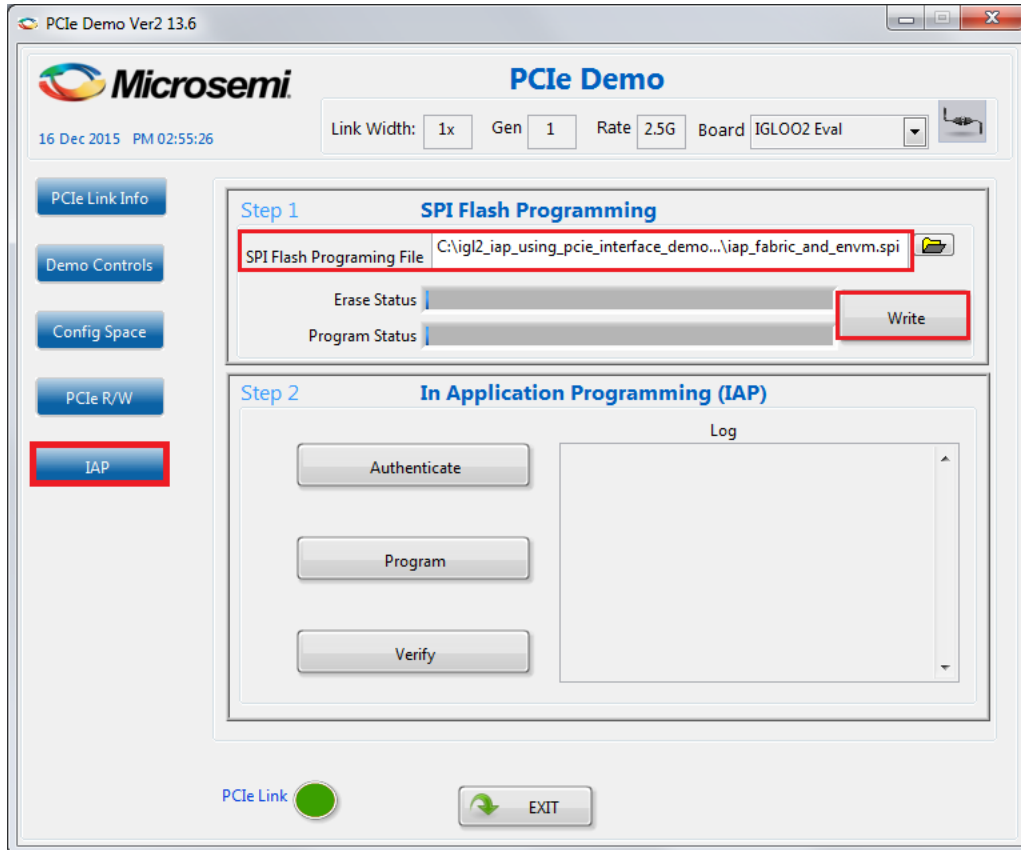
Figure 21 • Selecting Programming File
