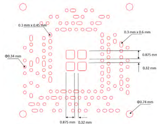
Figure 4 • Stencil Design
