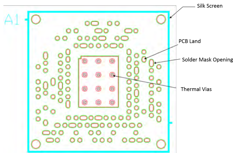
Figure 3 • PCB Land Pattern
