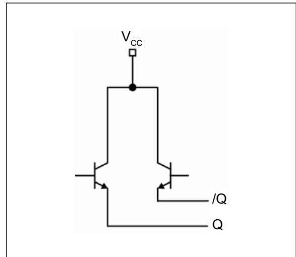
FIGURE 5-4: Simplified LVPECL Output Buffer.
