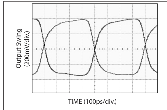
FIGURE 2-11: 1.25 GHz Clock.
