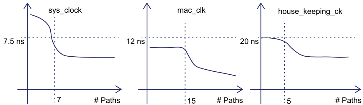
Figure 1 • Clock Domains and Slack Distribution Charts
