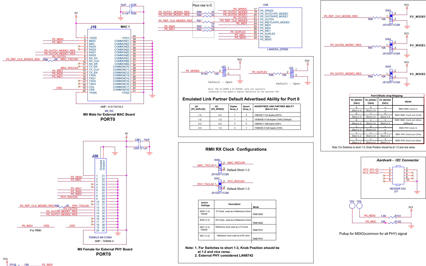
FIGURE B-7: EVB-LAN9354 EVALUATION BOARD SCHEMATIC 7
