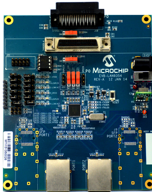
FIGURE A-1: EVB-LAN9354 EVALUATION BOARD
