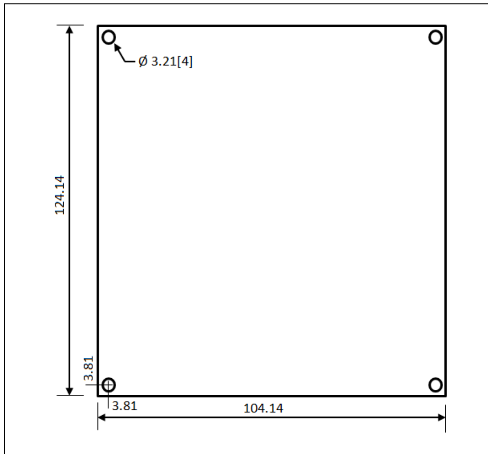
FIGURE 3-2: LAN9354 EVB MECHANICAL DIMENSIONS
