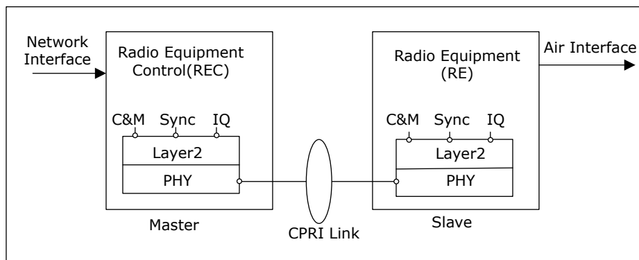
Figure 1-1. Radio Base Station System
