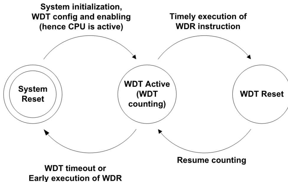
Figure 1-4. State Chart for Enabling WD through Fuses
