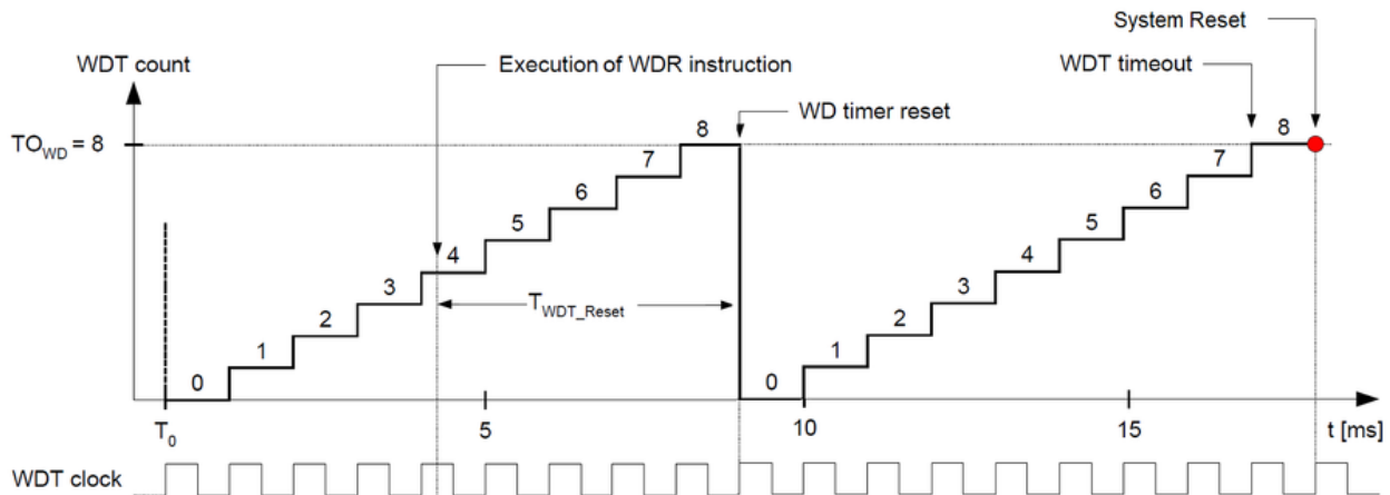
Figure 1-3. Digital Timing of the XMEGA Watchdog Timer
