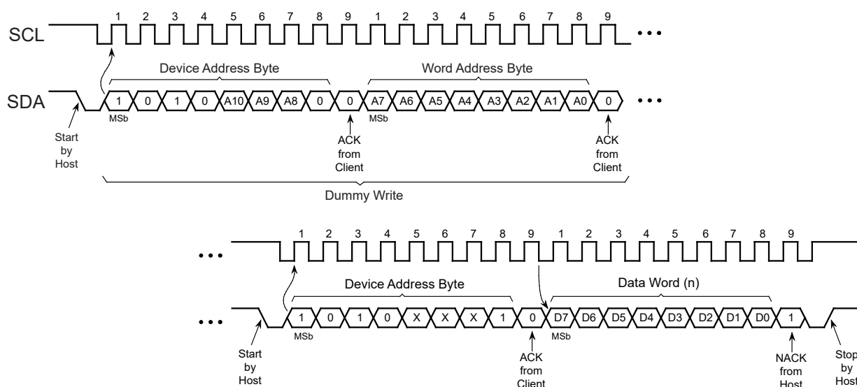
Figure 8-2. Random Read
