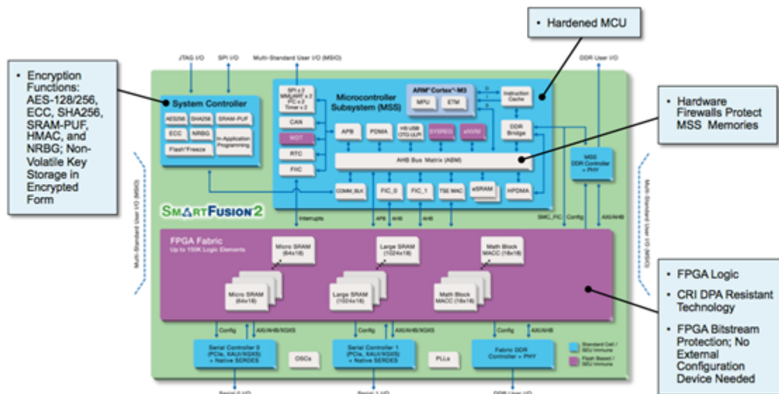
Figure 1: SmartFusion2 Architecture Block Diagram
