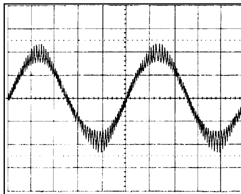
Figure 8: Voltage across C1 (100V/div, 500 us/div)
