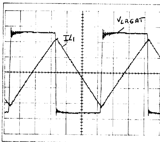
Figure 12. Module voltage and current (100V/div, 20A/div, 5us/div)
