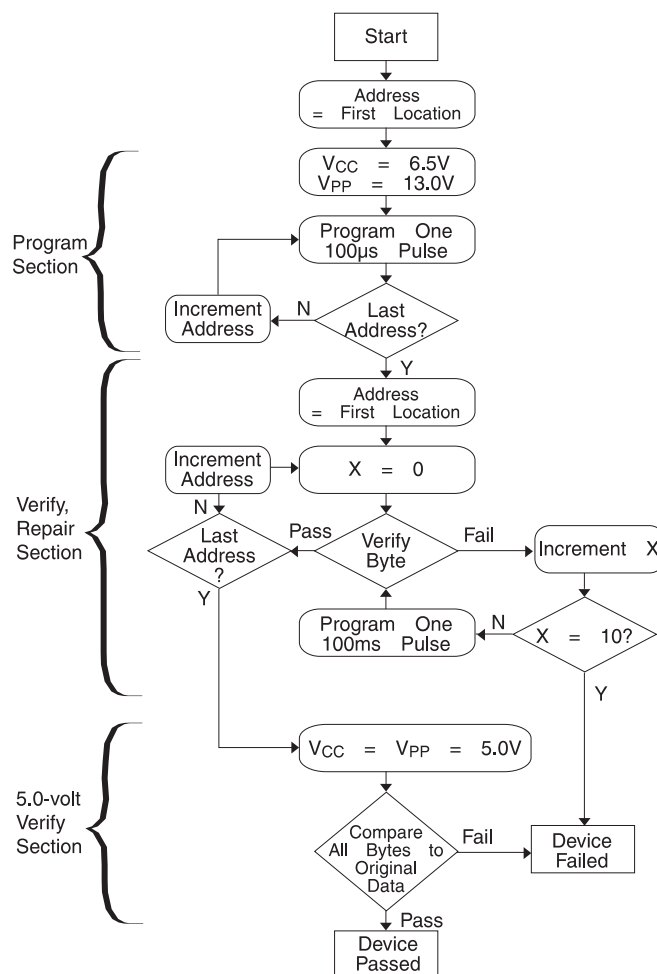
Figure 7. RAPID Programming Algorithm
