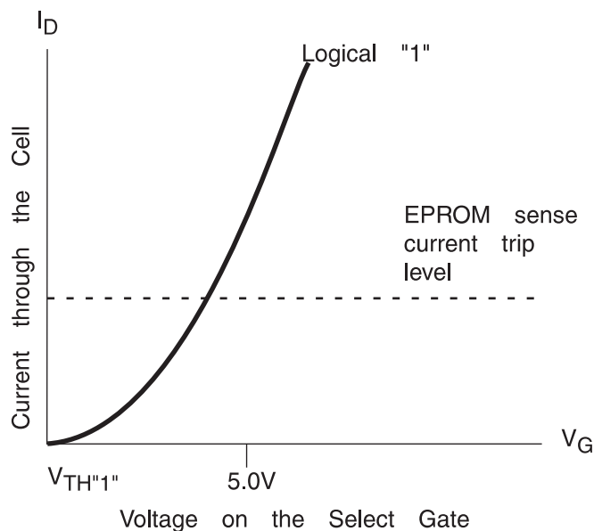
Figure 3. Unprogrammed Cell
