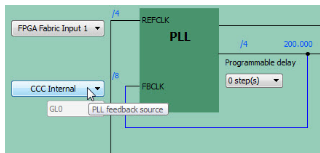
Figure 1-13 • PLL Feedback Source
