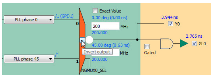
Figure 1-10 • Inverted Configuration
