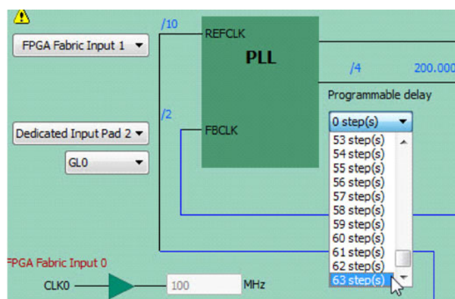
Figure 1-15 • Programmable Delay Line
