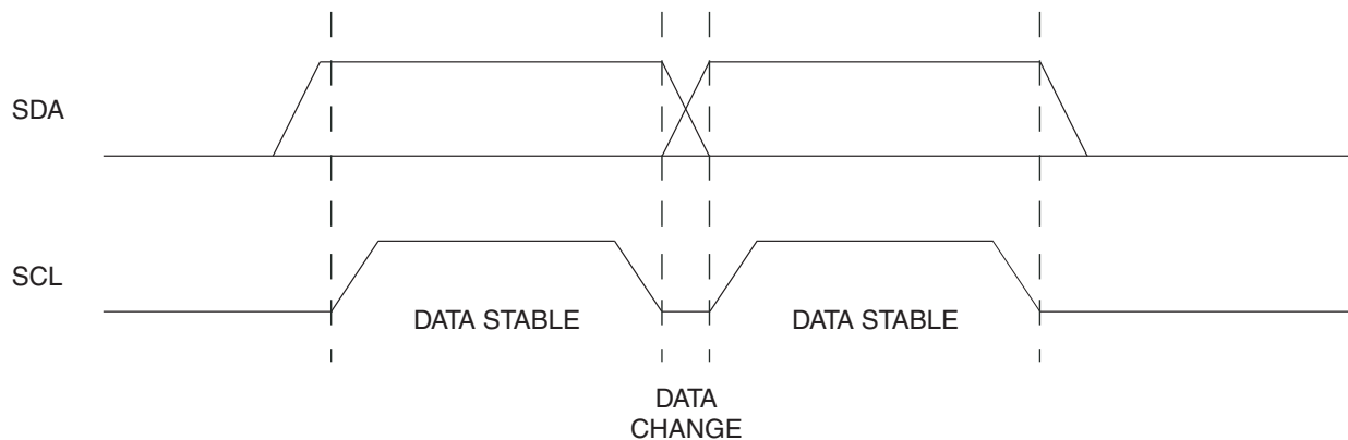
Figure 6-1. Two-Wire Protocol Timing - Data Validity
