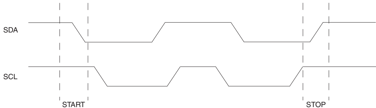
Figure 6-2. Two-Wire Protocol Timing - Start and Stop Definition
