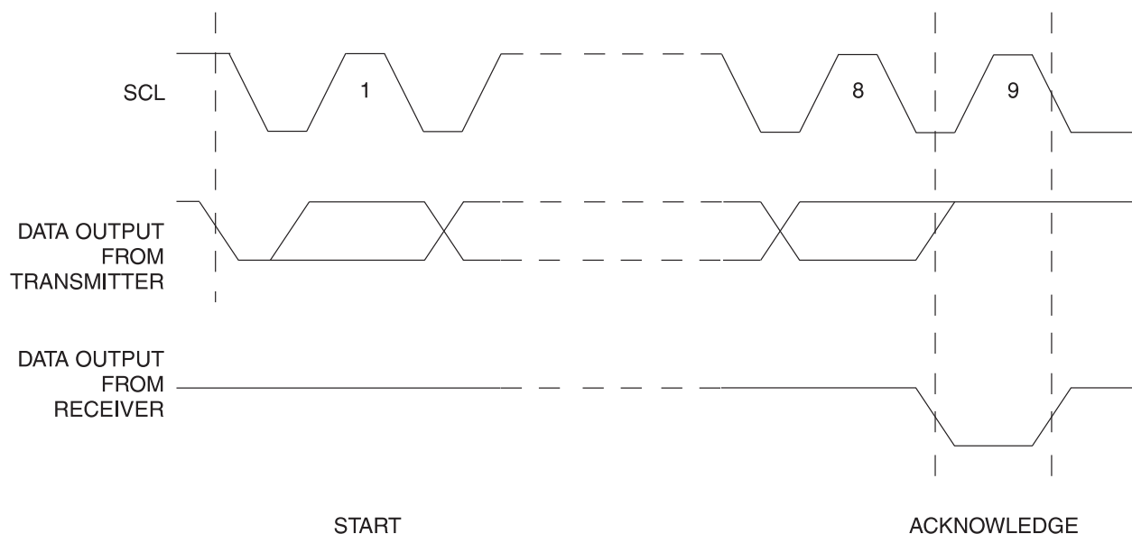
Figure 6-3. Two-Wire Protocol Timing - Acknowledge Response from Receiver
