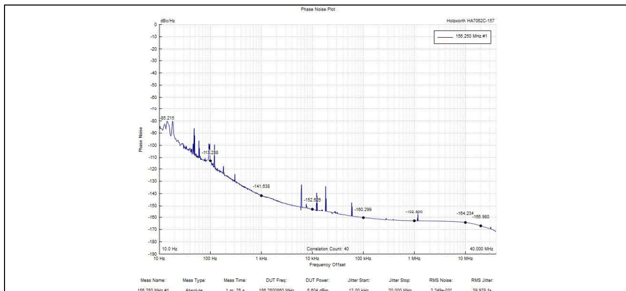
FIGURE 0-1: RMS Jitter, 40 fs RMS over 12 kHz to 20 MHz at 156.25 MHz.
