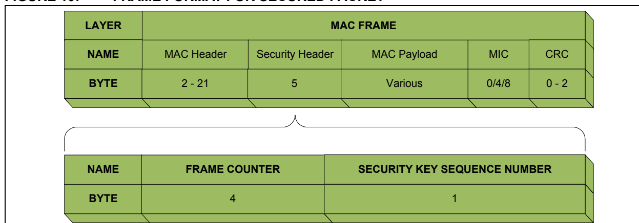
FIGURE 10: FRAME FORMAT FOR SECURED PACKET
