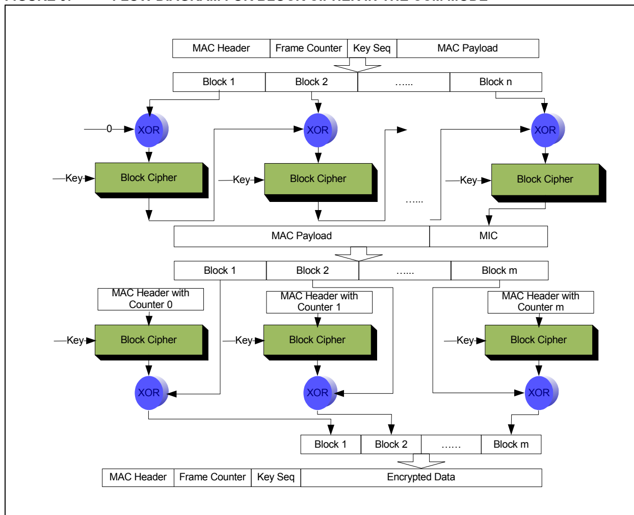
FIGURE 9: FLOW DIAGRAM FOR BLOCK CIPHER IN THE CCM MODE
