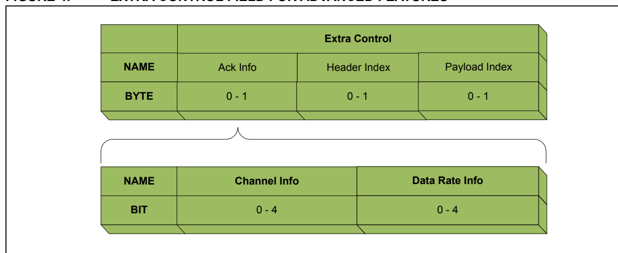
FIGURE 4: EXTRA CONTROL FIELD FOR ADVANCED FEATURES
