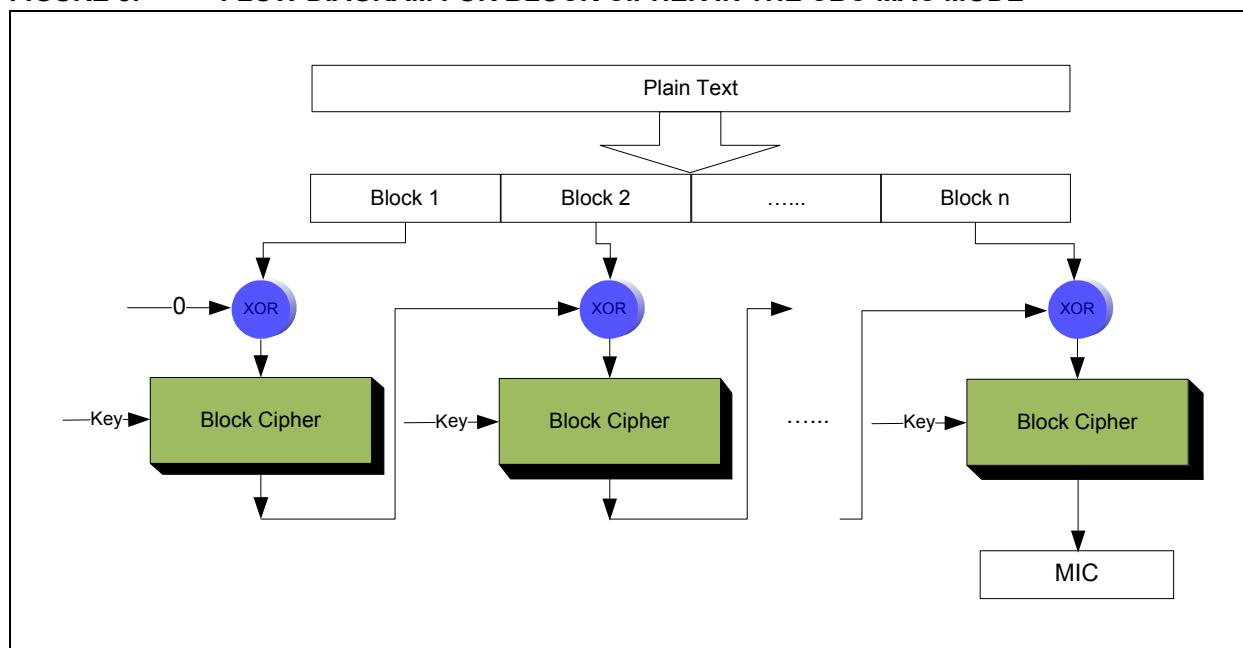
FIGURE 8: FLOW DIAGRAM FOR BLOCK CIPHER IN THE CBC-MAC MODE
