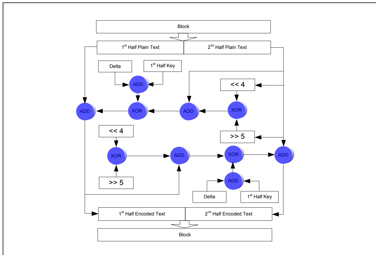
FIGURE 5: BLOCK DIAGRAM OF XTEA CIPHER
