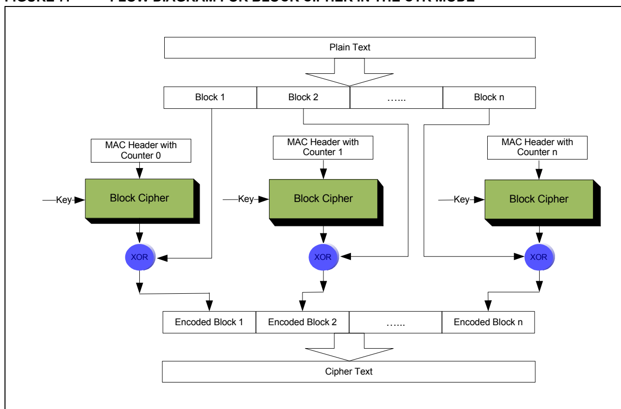
FIGURE 7: FLOW DIAGRAM FOR BLOCK CIPHER IN THE CTR MODE
