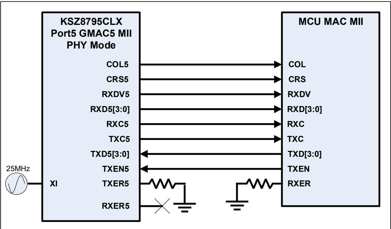
FIGURE 7-2: CONNECTIONS BETWEEN KSZ8795CLX PORT 5 GMAC5 MII PHY MODE AND MCU MAC MII
