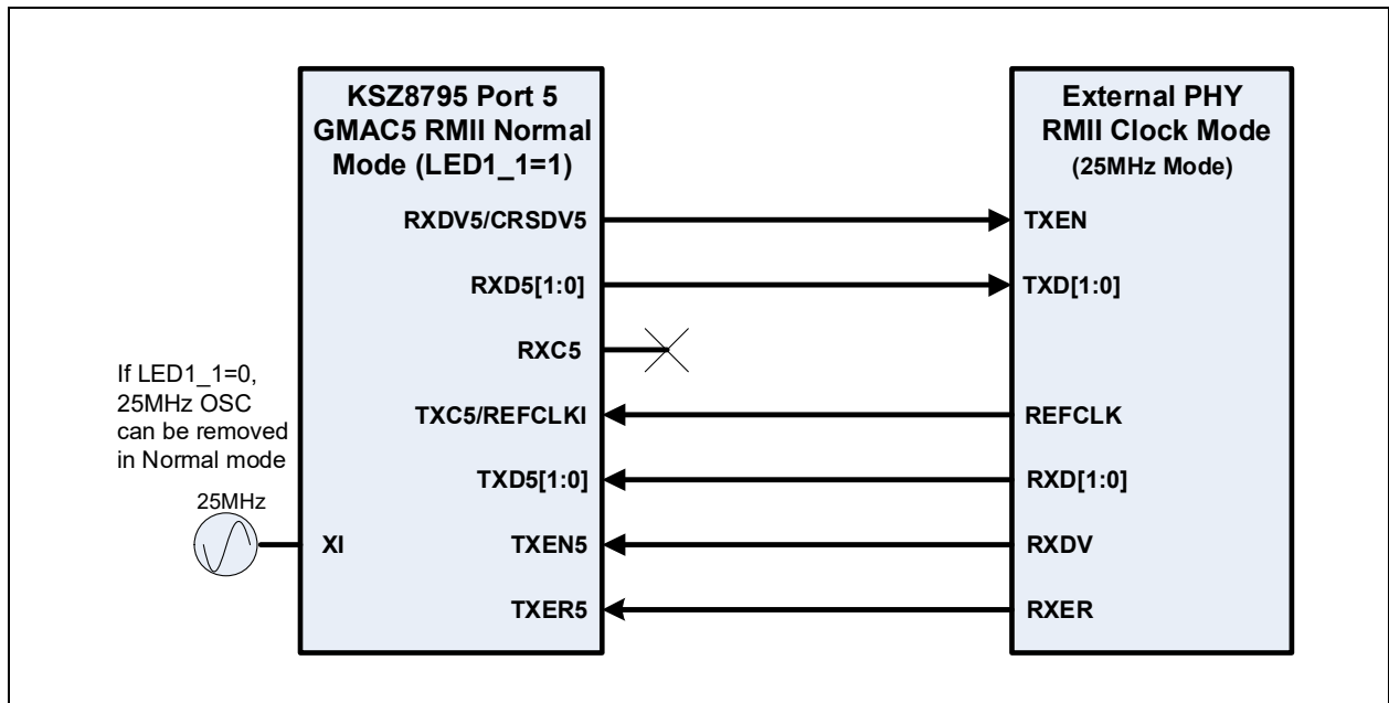
FIGURE 7-6: CONNECTIONS BETWEEN KSZ8795CLX PORT 5 RMII NORMAL MODE AND EXTERNAL PHY RMII™ CLOCK MODE
