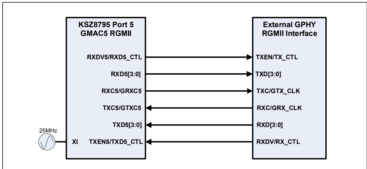
FIGURE 7-10: CONNECTIONS BETWEEN KSZ8795CLX PORT 5 RGMII AND A GPHY RGMII INTERFACE
