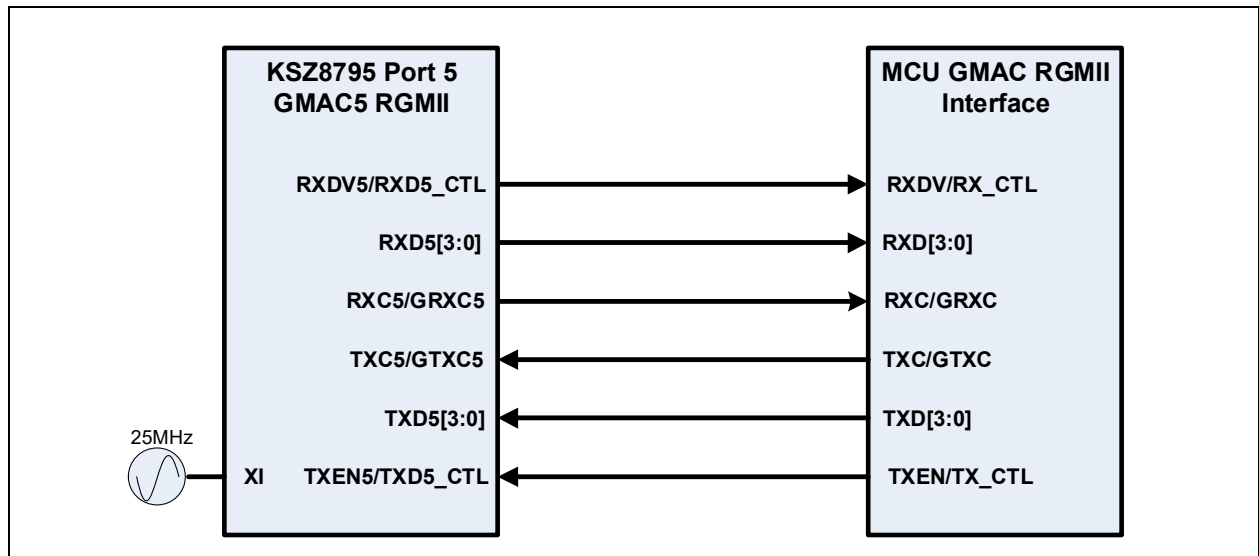
FIGURE 7-9: CONNECTIONS BETWEEN KSZ8795CLX PORT 5 RGMII AND MCU GMAC RGMII INTERFACE
