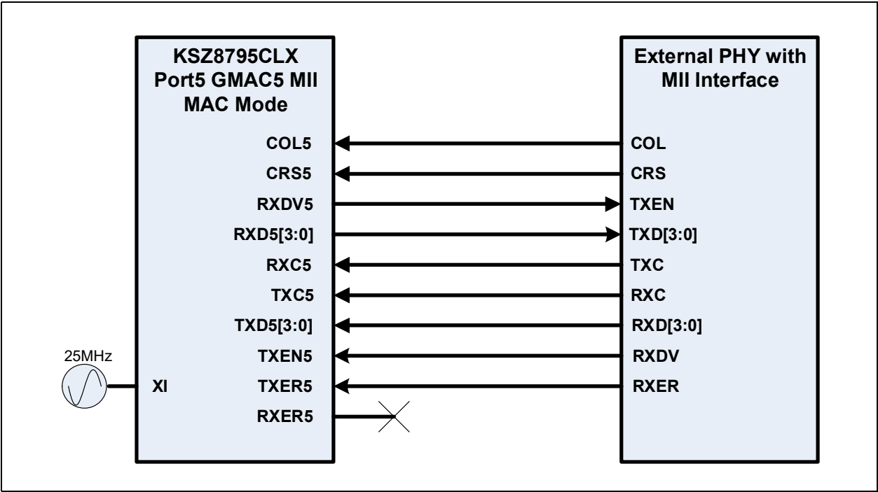
FIGURE 7-1: CONNECTIONS BETWEEN KSZ8795CLX PORT 5 GMAC5 MII MAC MODE AND EXTERNAL PHY WITH MII INTERFACE
