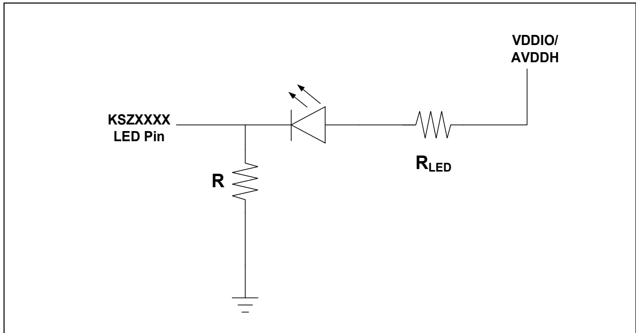
FIGURE 10-1: CONNECTION WHEN LED STRAP PIN IS USED FOR A STRAP-LOW
