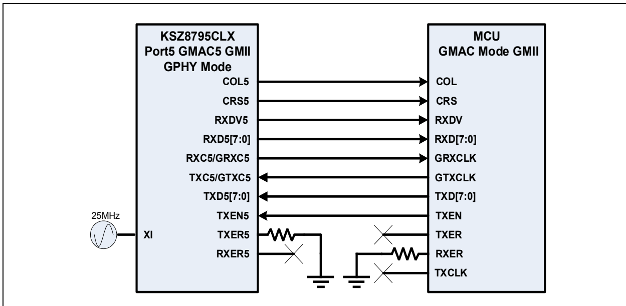
FIGURE 7-8: CONNECTIONS BETWEEN KSZ8795CLX PORT5 GMAC5 GMII GPHY MODE AND MCU GMAC GMII INTERFACE
