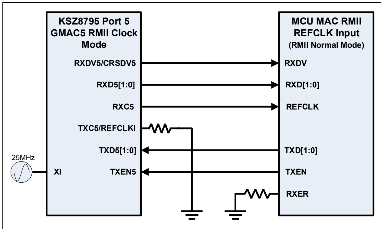
FIGURE 7-3: PORT 5 GMAC5 RMII™ CLOCK MODE AND MCU MAC RMII REFCLK INPUT MODE
