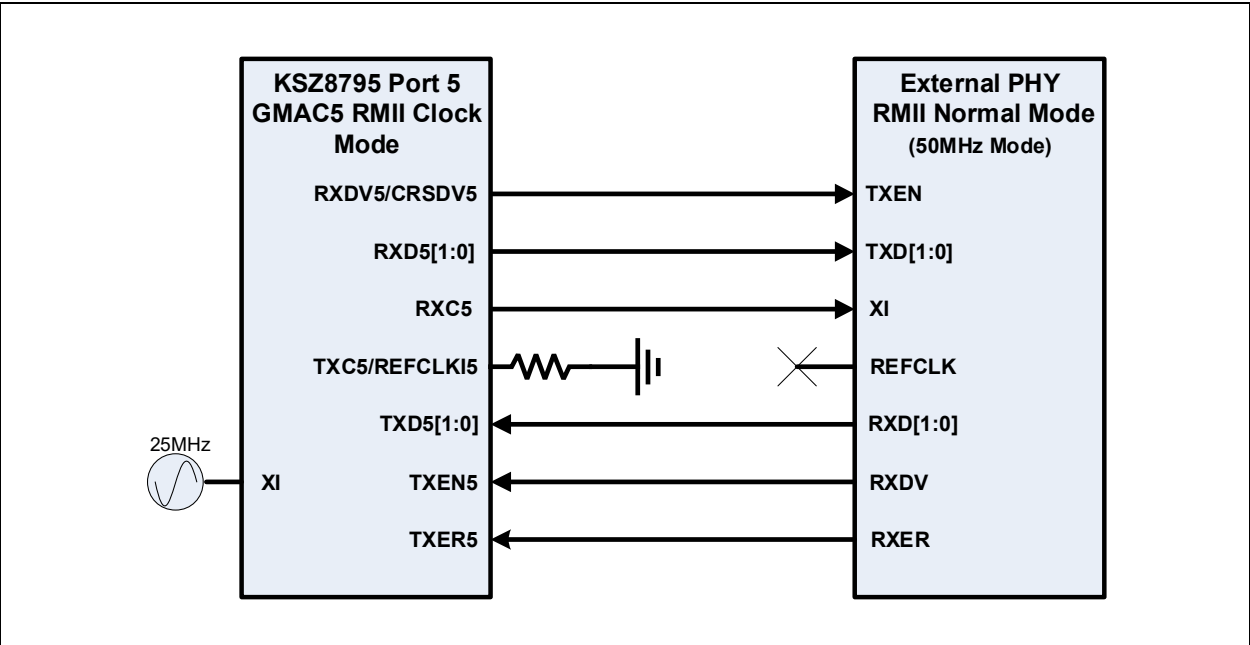
FIGURE 7-4: PORT 5 GMAC5 RMII™ CLOCK MODE AND EXTERNAL PHY RMII NORMAL MODE
