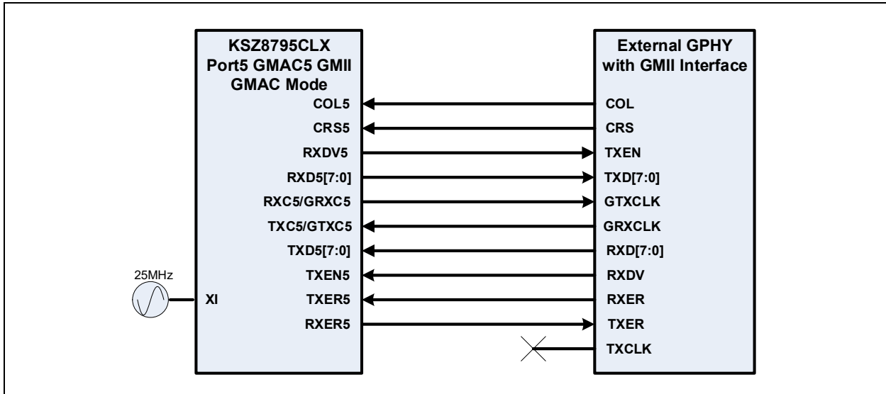
FIGURE 7-7: CONNECTIONS BETWEEN KSZ8795CLX PORT 5 GMII GMAC MODE AND EXTERNAL GPHY GMII INTERFACE
