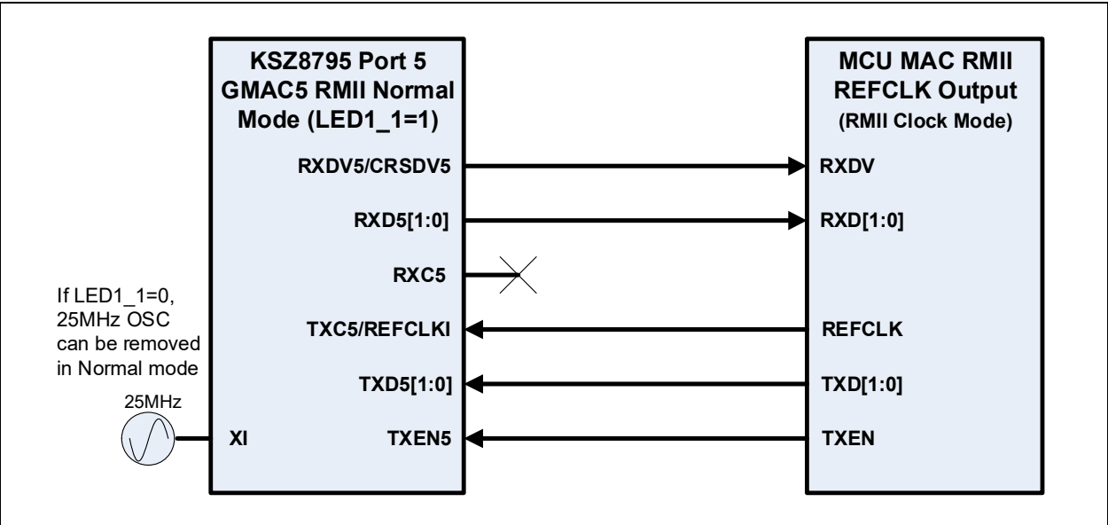
FIGURE 7-5: CONNECTIONS BETWEEN KSZ8795CLX PORT 5 RMII™ NORMAL MODE AND MCU RMII REFCLK OUTPUT MODE
