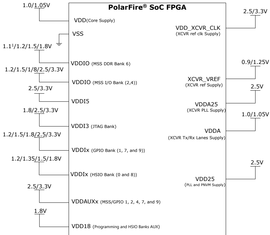
Figure 1-1. Power Supplies
