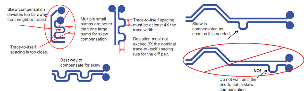
Figure 3-2. Skew Matching
