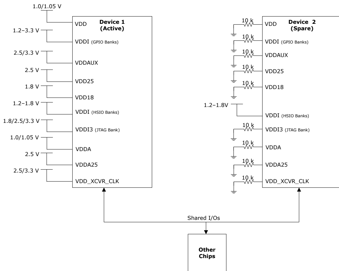
Figure 1-4. Cold Sparing
