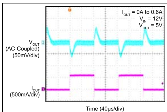
FIGURE 2-56: MIC28512-2 Load Transient Response (0A to 0.6A).
