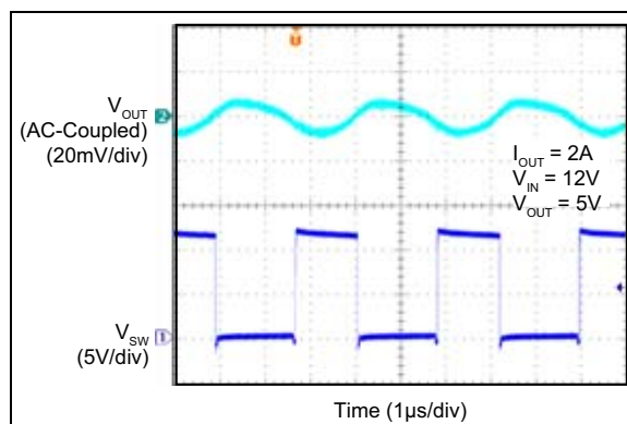
FIGURE 2-52: MIC28512-2 Switching Waveform ( I_{OUT} = 2A ).
