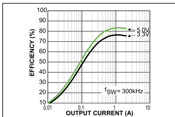
FIGURE 2-19: Efficiency ( V_{IN} = 48V ) vs. Output Current (MIC28512-2).
