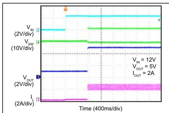
FIGURE 2-31: V_{IN} Start-Up with 1V Pre-Biased Output (MIC28512-2).
