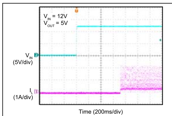
FIGURE 2-33: Start-Up Into Short Circuit (MIC28512-2).
