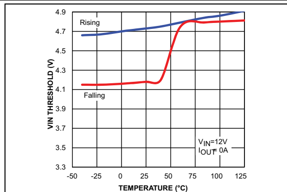
FIGURE 2-4: V_{IN} ULVO Threshold vs. Temperature.
