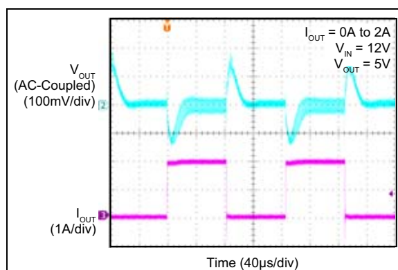
FIGURE 2-54: MIC28512-2 Load Transient Response (0A to 2A).
