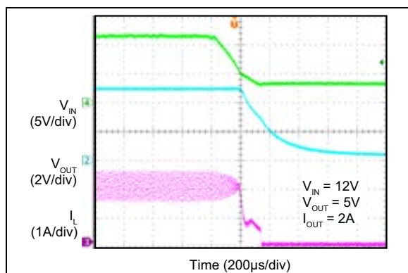
FIGURE 2-44: V_{IN} Shutdown (MIC28512-1).
