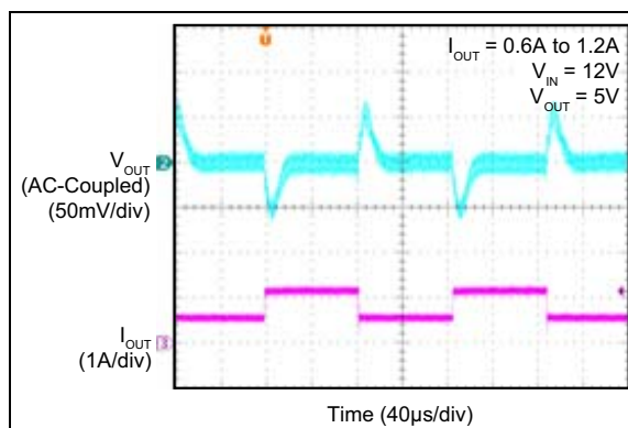
FIGURE 2-58: MIC28512-2 Load Transient Response (0.6A to 1.2A).
