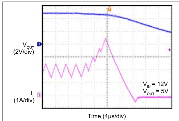
FIGURE 2-35: Inductor Peak Current (Output Short Applied) (MIC28512-2).
