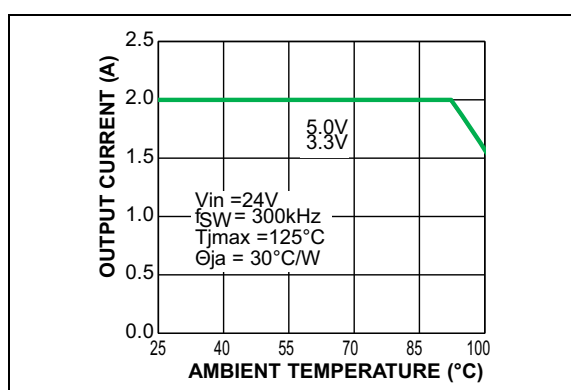
FIGURE 2-24: 24V Input Thermal Derating.
