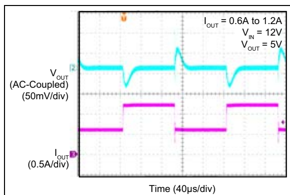
FIGURE 2-55: MIC28512-1 Load Transient Response (0A to 0.6A).
