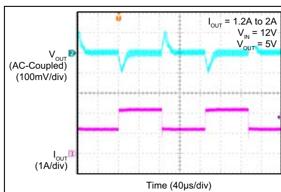
FIGURE 2-60: MIC28512-2 Load Transient Response (1.2A to 2A).
