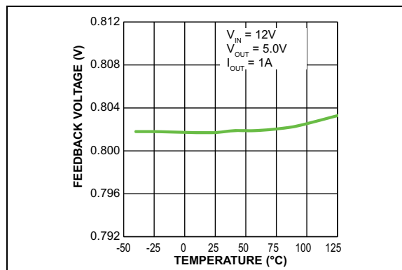
FIGURE 2-6: Feedback Voltage vs. Temperature (MIC28512-1).
