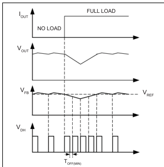
FIGURE 4-3: MIC28512 Load Transient Response.
