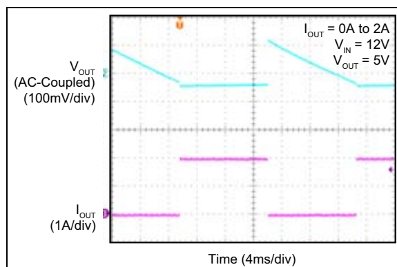
FIGURE 2-53: MIC28512-1 Load Transient Response (0A to 2A).
