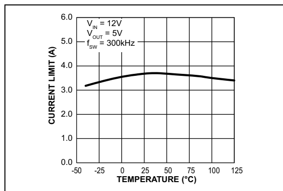
FIGURE 2-5: Output Peak Current Limit vs. Temperature.
