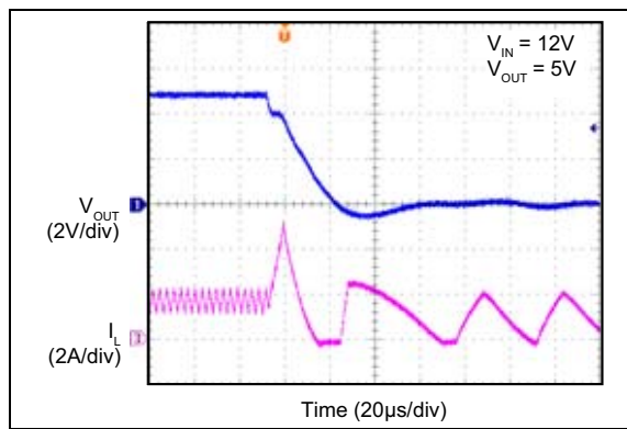
FIGURE 2-36: Short Circuit (MIC28512-2).
