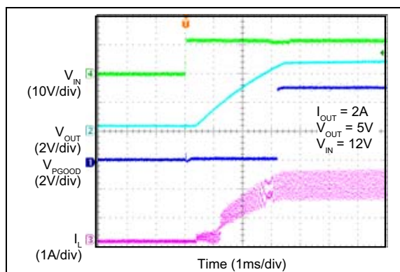
FIGURE 2-46: Soft Start Power Good (MIC28512-1).
