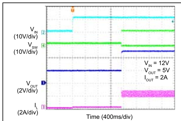
FIGURE 2-32: V_{IN} Start-Up with 2V Pre-Biased Output (MIC28512-2).
