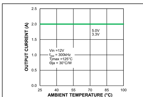
FIGURE 2-23: 12V Input Thermal Derating.
