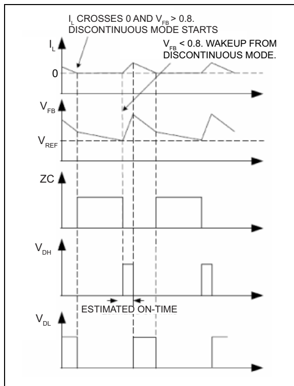
FIGURE 4-4: MIC28512-1 Control Loop Timing (Discontinuous Mode).
