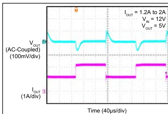
FIGURE 2-59: MIC28512-1 Load Transient Response (1.2A to 2A).
