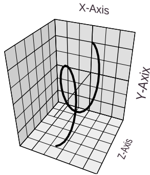
Figure 5c. Elliptical Polarization
