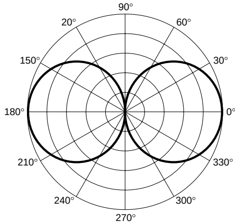
Figure 6. 0.25\lambda Monopole Over Ground Plane
